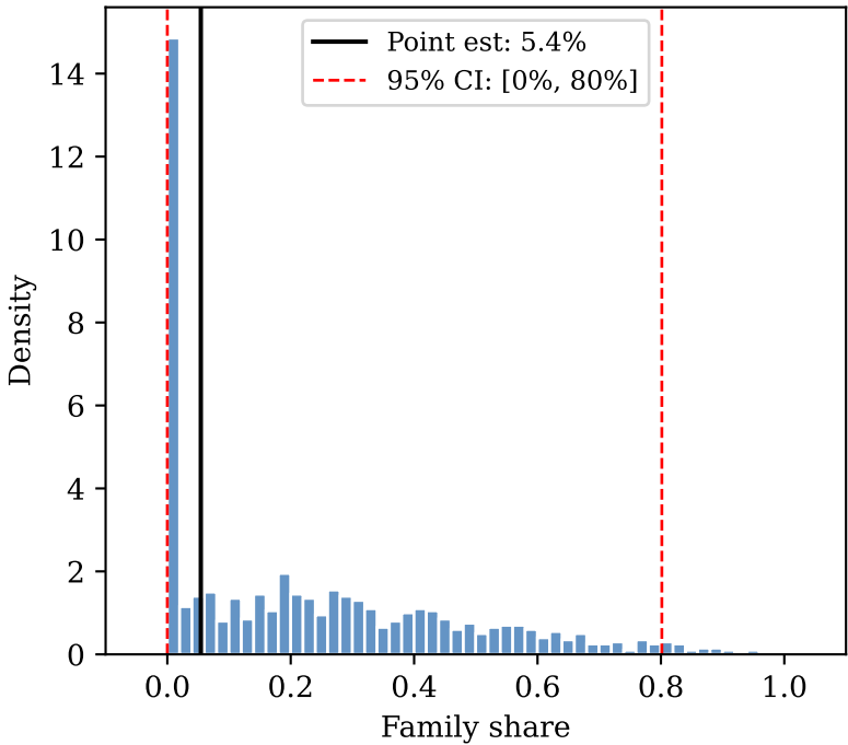
(b) Bootstrap Distribution (Uninformative)
