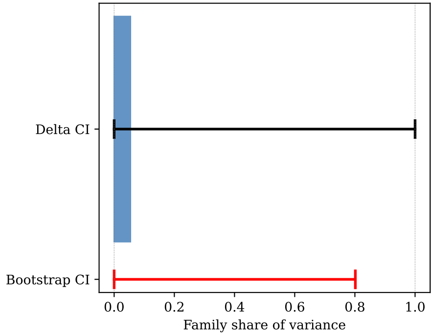
(a) Family Share \hat{\theta}_p (DIAGNOSTIC ONLY)
