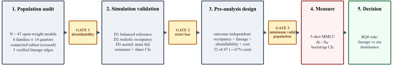
FIGURE 2. Protocol architecture. Three completed stages (population audit, simulation validation, pre-analysis study-population design), each behind an identifiability or recoverability gate, followed by the measurement and decomposition stage the instrument gates and the decision layer. Stages 1–3 constitute the instrument and are established in this paper; stage 4 is specified in full by the pre-registered protocol of Section V-E. The G3 stage is outcome-independent: it never observes trait values.
