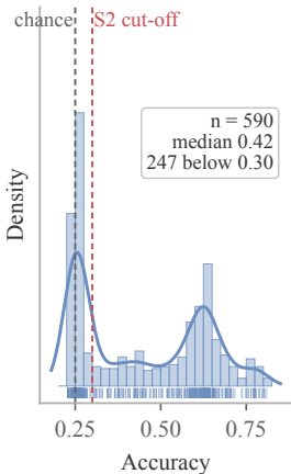
(a) Distribution
