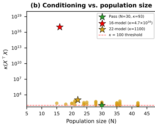
FIGURE 9: Conditioning versus population size. The condition number \kappa is shown for all full-rank designs, with the \kappa = 100 numerical-gate threshold marked. The passing design (N = 30, \kappa = 93 ) sits below the threshold; the measured 16-model population ( \kappa = 4.7 \times 10^{16} ) and the 22-model candidate ( \kappa = 1100 ) are noted as reference points.
