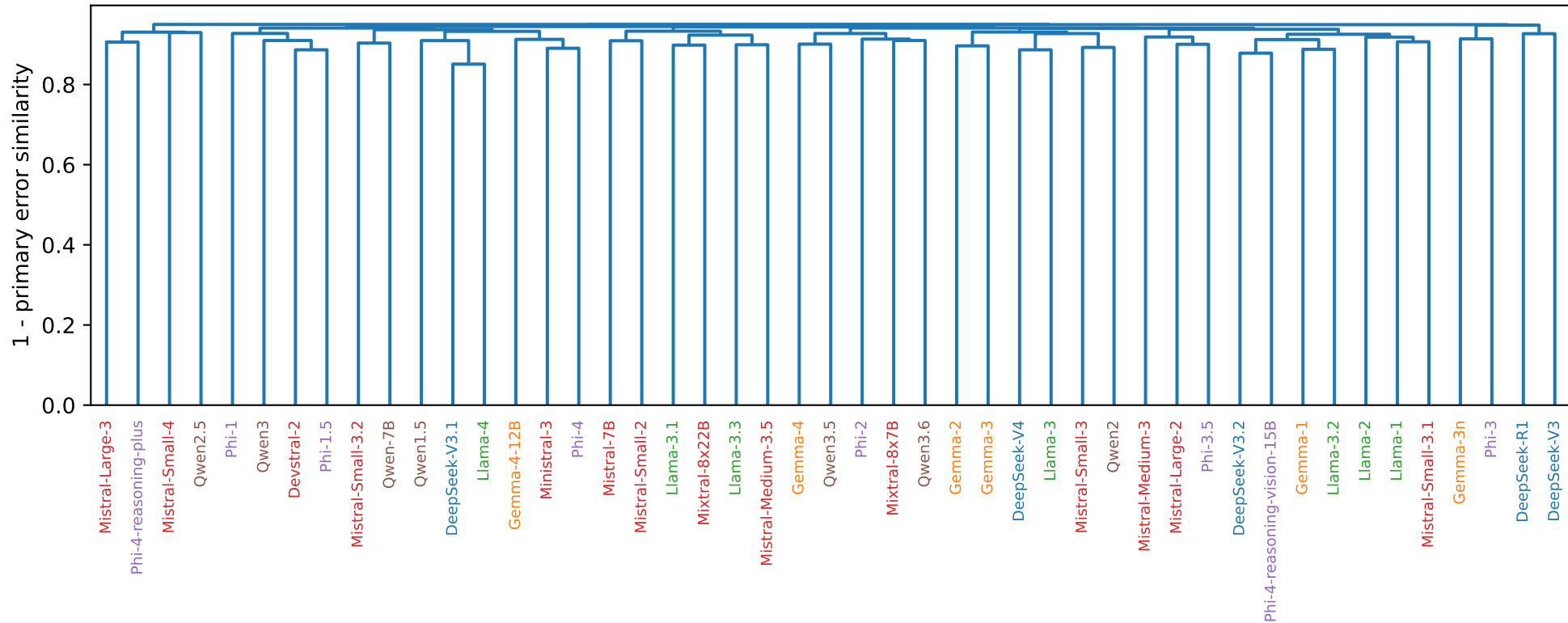
Average-linkage clustering of models by error similarity
