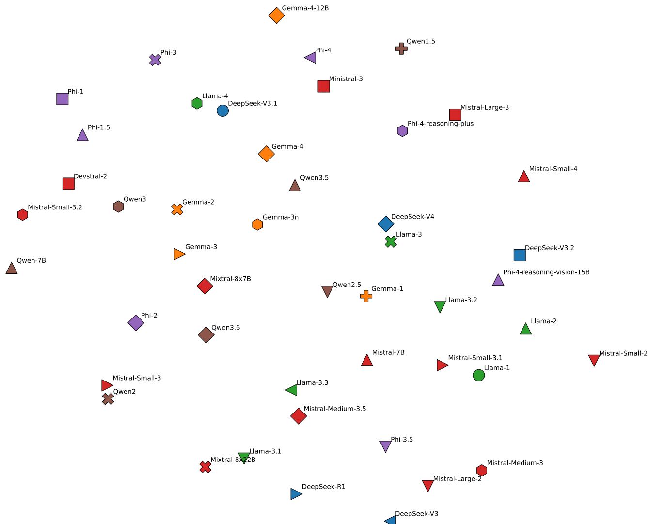
Model error-similarity: t-SNE (color=family, marker=era)
