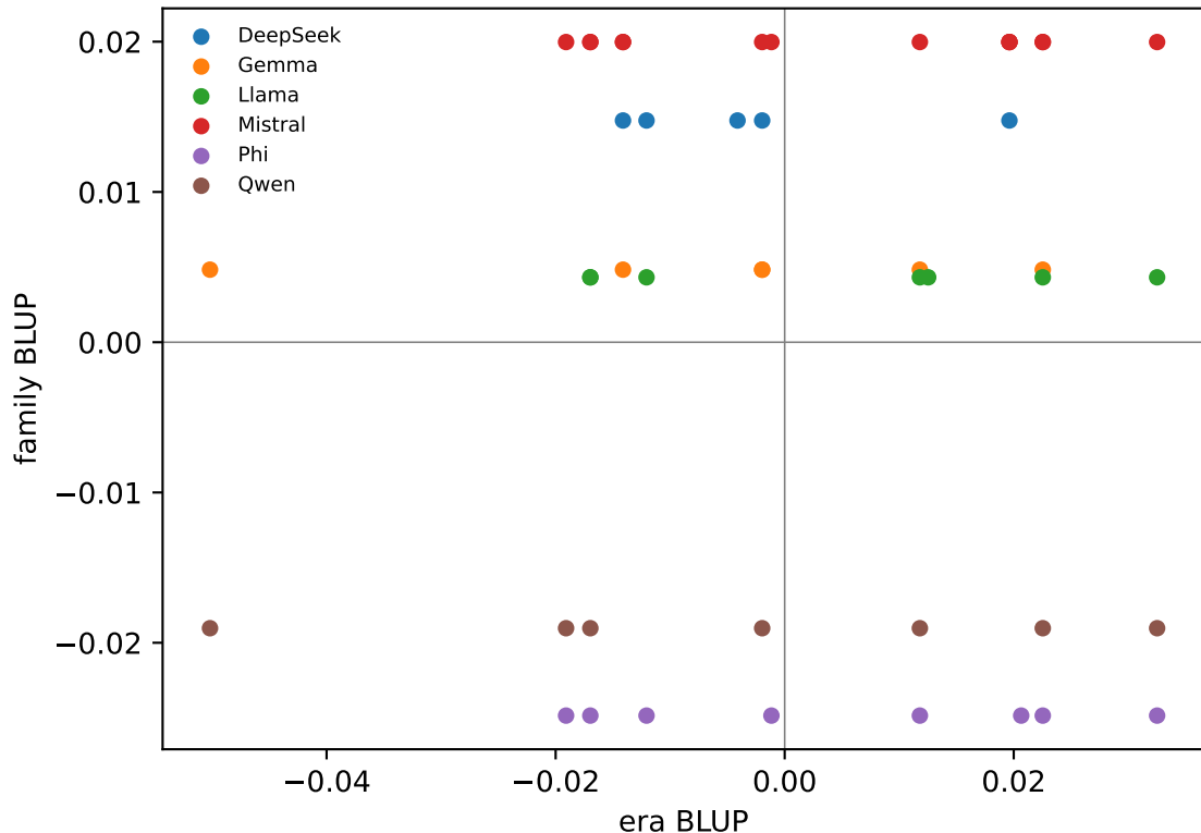
Per-model family vs era BLUPs (alias check)
