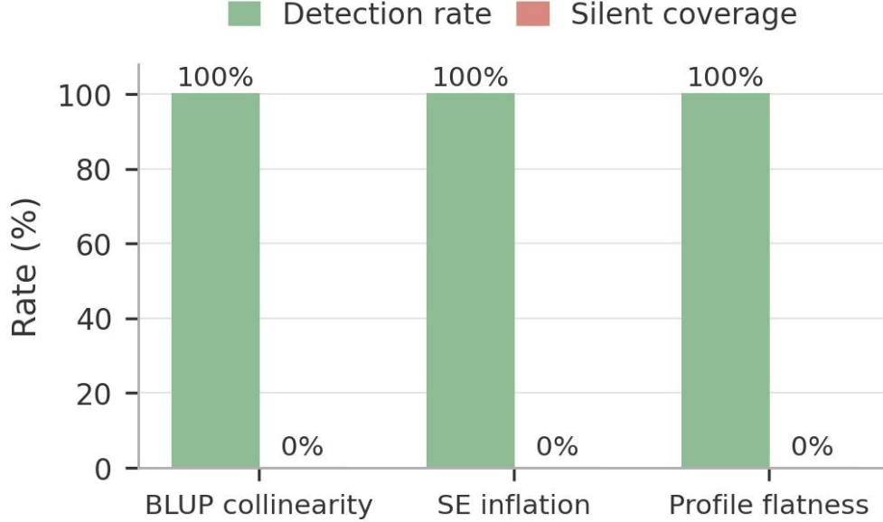
Figure 5. D3 failure detection. Three complementary failure detectors (BLUP collinearity, SE inflation, profile flatness) flag nested aliasing in 100% of repetitions with zero silent coverage across all scenarios.
