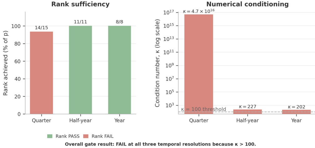
Figure 15. Era-resolution sensitivity. Gate diagnostics at quarter, half-year, and year resolution. Collapsing quarters eliminates rank deficiency but does not satisfy the numerical stability gate: \kappa remains above 100 at all resolutions.
