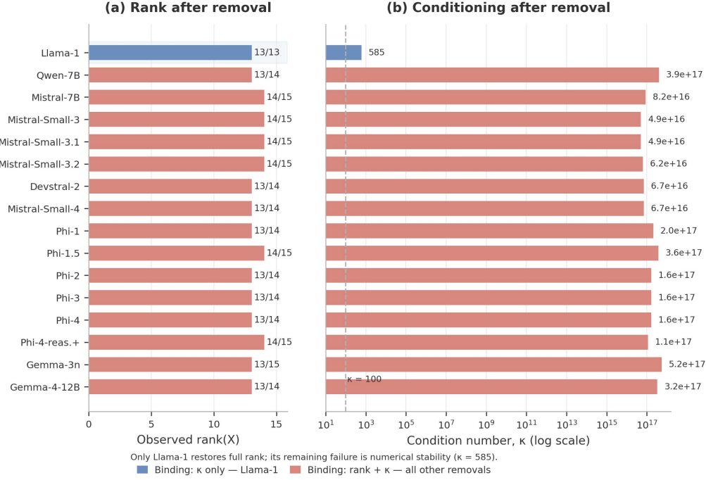
Figure 14. Leave-one-model-out diagnostics. Each row shows the rank and condition number after removing one model. Removing Llama-1 alone restores full rank (13/13) but \kappa = 585 > 100 , demonstrating that rank deficiency and conditioning failure are separable problems.
