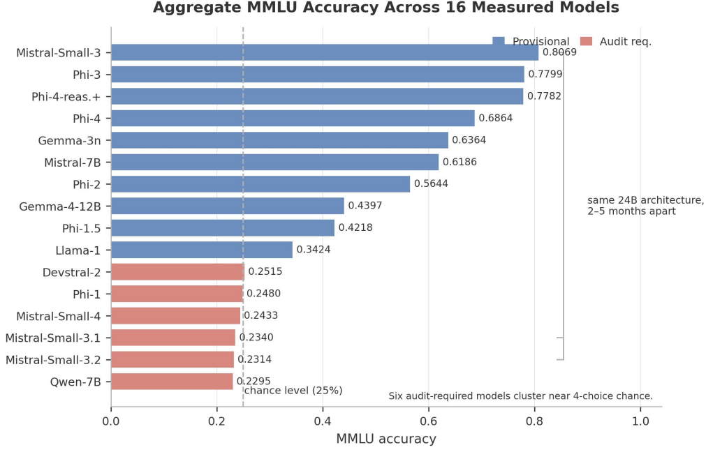
Figure 7. Distribution of measured MMLU accuracy (provisional). These are descriptive aggregate values reported for diagnostic context only; their evaluation validity is pending an independent audit because the recorded per-question answers were non-informative (Sec. 11). Six models cluster near the chance level (23–25%) for a 4-choice benchmark, triggering an evaluation-validity audit. The identifiability gate is invariant to accuracy values.
