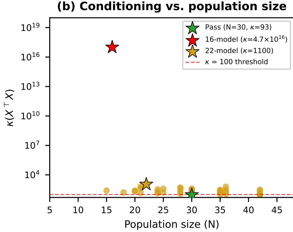
Figure 11. Conditioning versus population size. The condition number \kappa is shown for all full-rank designs, with the \kappa = 100 numerical-gate threshold marked. The passing design (N = 30, \kappa = 93 ) sits below the threshold; the measured 16-model population ( \kappa = 4.7 \times 10^{16} ) and the 22-model candidate ( \kappa = 1100 ) are noted as reference points.
