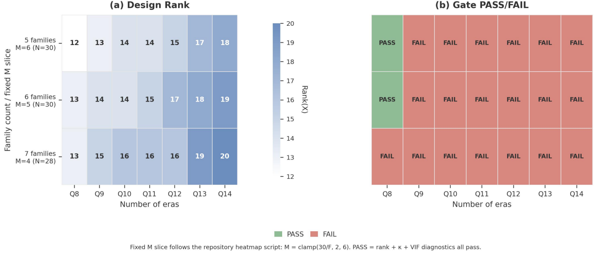
Figure 13. PASS/FAIL heatmap across the design space. Each cell shows whether a given (N, F, E) configuration passes all three numerical/design-matrix diagnostics: full rank, \kappa \leq 100 , and \text{VIF} \leq 10 . Crossing and connectedness are enforced by the staggered assignment constraints.
