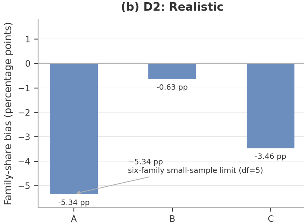
Figure 3. Simulation recovery: D2 family-share bias. Each bar reports the signed family-share bias (\hat{s}_{\text{family}} - s_{\text{family}}) \times 100 pp under the realistic sparse D2 occupancy (47-model occupancy, 300 repetitions). The -5.3 pp family-share bias in scenario A is the documented six-family small-sample limit ( df = 5 ).
