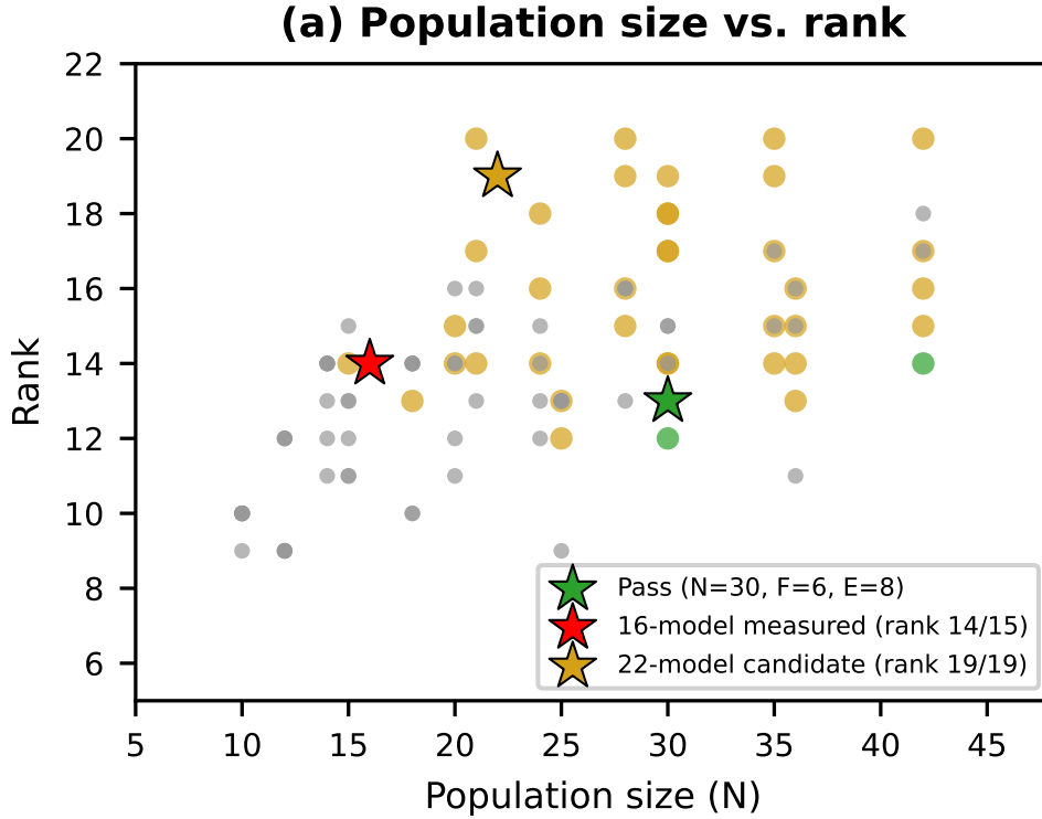
Figure 10. Population size versus rank across the design space. Each point is one evaluated (F, E, M) configuration. The passing design ( N = 30 , F = 6 , E = 8 ) is highlighted; the measured 16-model population (rank 14/15) and the 22-model candidate (rank 19/19) are marked as reference points.
