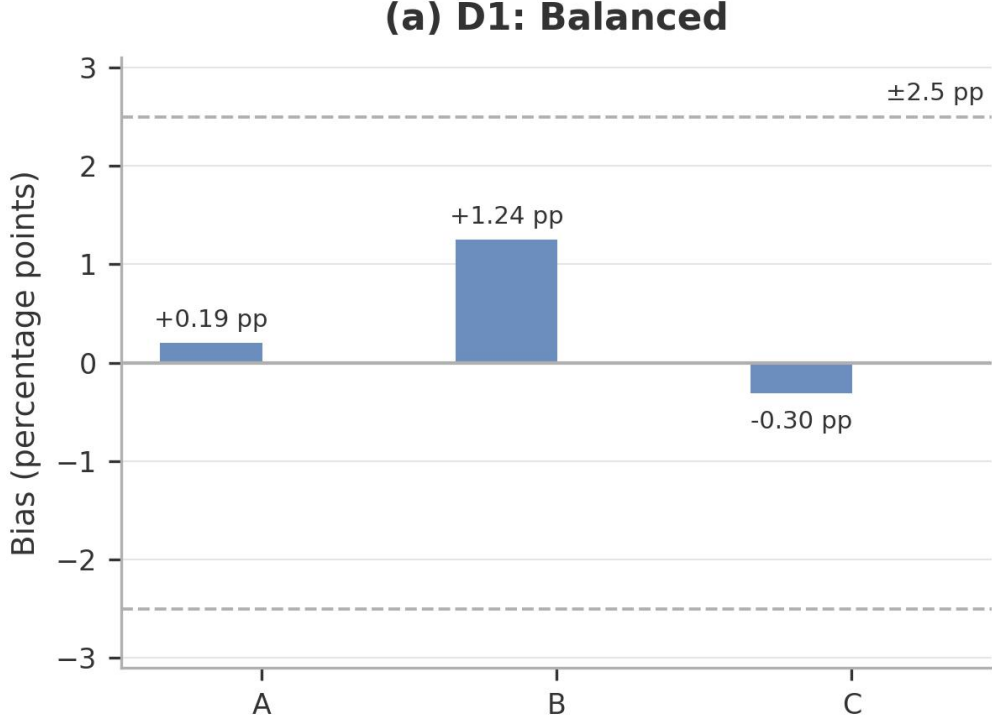
Figure 2. Simulation recovery: D1 family-share bias. Each bar reports the signed family-share bias (\hat{s}_{\text{family}} - s_{\text{family}}) \times 100 pp, averaged over converged repetitions, for the balanced crossed reference regime D1 (30 families \times 14 eras \times 2 models, 300 repetitions). Family-share-bias panels are recovery diagnostics; the selection acceptance criterion in Algorithm 1 uses era-share bias, whose values for the 22-model selection are reported in TABLE IV.
