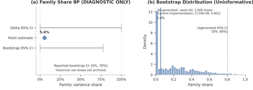
Figure 16. Diagnostic variance-component estimates under the invalid (non-identifiable) 16-model design. Panel (a): historical bootstrap interval as originally reported (raw draws not archived). Panel (b): regenerated sensitivity analysis for reference only — NOT the primary result. The 95% confidence interval for the family share covers [0%, 100%], reflecting the non-identifiability of the rank-deficient design. The near-zero era estimate is an aliasing artifact, not evidence of no era effect. These estimates are not scientifically interpretable.
