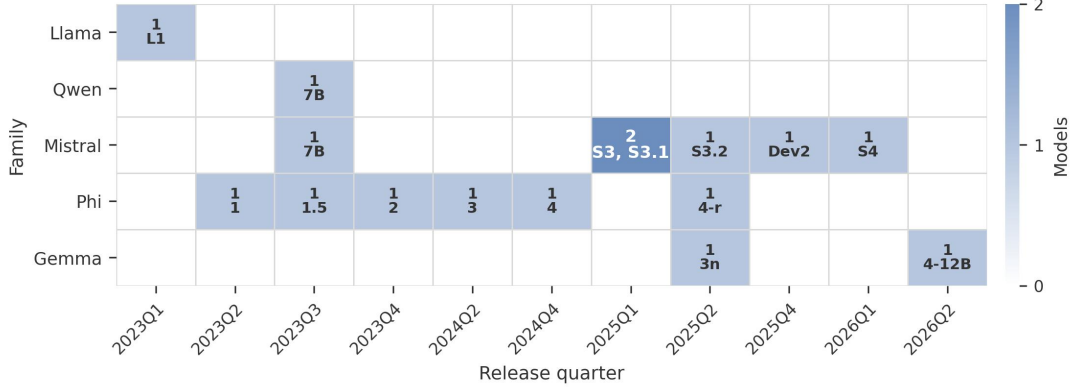
Figure 8. Family×era occupancy heatmap of the 16 measured models. Darker shading indicates more models in a cell. 8 of 11 occupied quarters contain only one model; 40 of 55 possible cells are empty (73% sparse).
