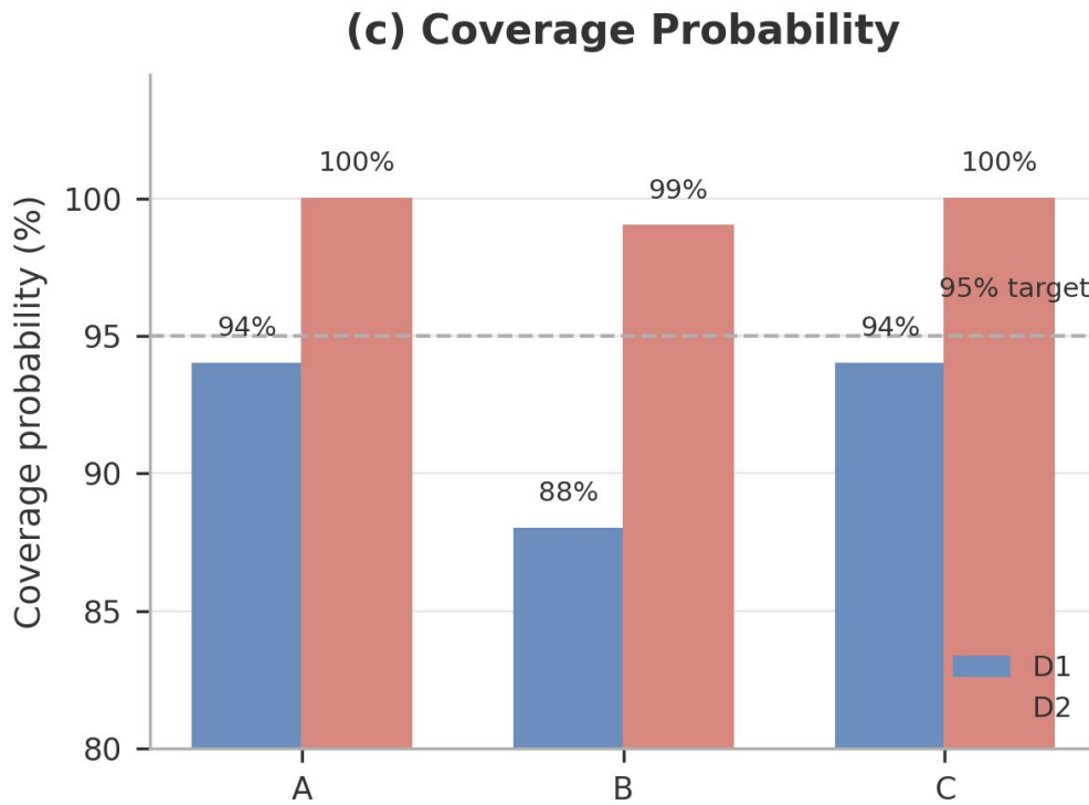
Figure 4. Simulation recovery: 95% CI coverage. Coverage of the 95% confidence intervals under the D1 (balanced crossed) and D2 (realistic occupancy) regimes across scenarios A–C.
