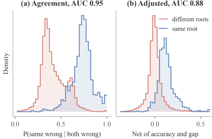
Figure S6: Agreement as a signal of shared lineage (primary sample; 2,020 same-root and 171,735 different-root pairs; densities). (a) Observed agreement on wrong answers. (b) Agreement after removing the accuracy and release-gap terms of the pre-specified model. AUC: probability that a random same-root pair scores higher than a random different-root pair.
