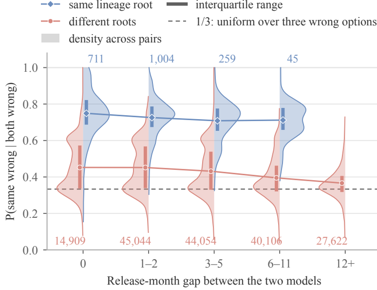
Figure 5. Agreement on wrong answers by release-month gap (primary sample, unadjusted). Half-violins: density across pairs (left, different roots; right, same root); markers: means; bars: interquartile ranges; labels: pairs. Dashed line: 1/3, uniform choice among three wrong options.
