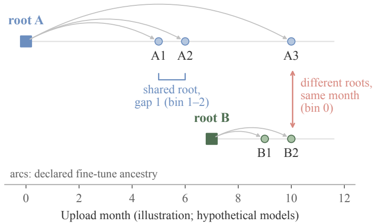
Figure 4. The two pair-level predictors (hypothetical models). Squares are lineage roots, circles fine-tunes at their upload month, arcs declared ancestry. A1 and A2 share a root, one month apart (gap bin 1–2); A3 and B2 have different roots, same month (gap bin 0). The outcome is agreement on wrong answers, adjusted for both accuracies.
