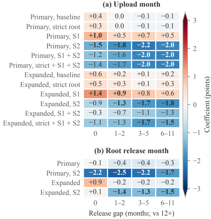
Figure 9. Release-gap coefficients (points, relative to a gap of 12+ months; bold: 95% CI excludes zero). (a) Upload month, all twelve analyses fixed before any pair outcome (model-level CIs, as in Table IV). (b) The roots’ release month in place of upload month (jackknife CIs).
