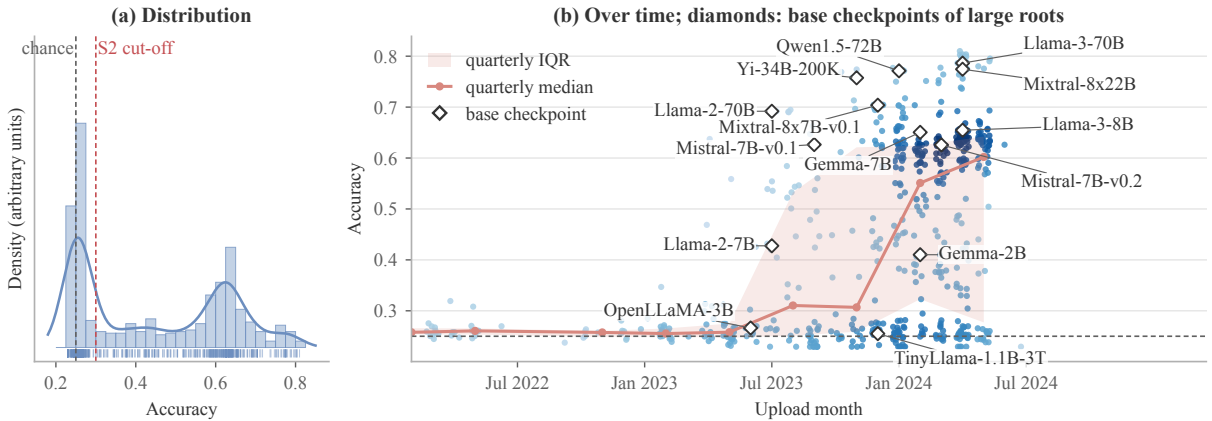
Figure 7. Model accuracy (primary sample; n = 590 , median 0.415, 247 below 0.30). (a) Histogram, kernel density and rug; dashed lines: chance (0.25) and the S2 cut-off (0.30). (b) By upload month, with the quarterly median and interquartile range (quarters with \geq 10 models; Spearman \rho = 0.41 ); diamonds: the base checkpoints of the largest roots.
