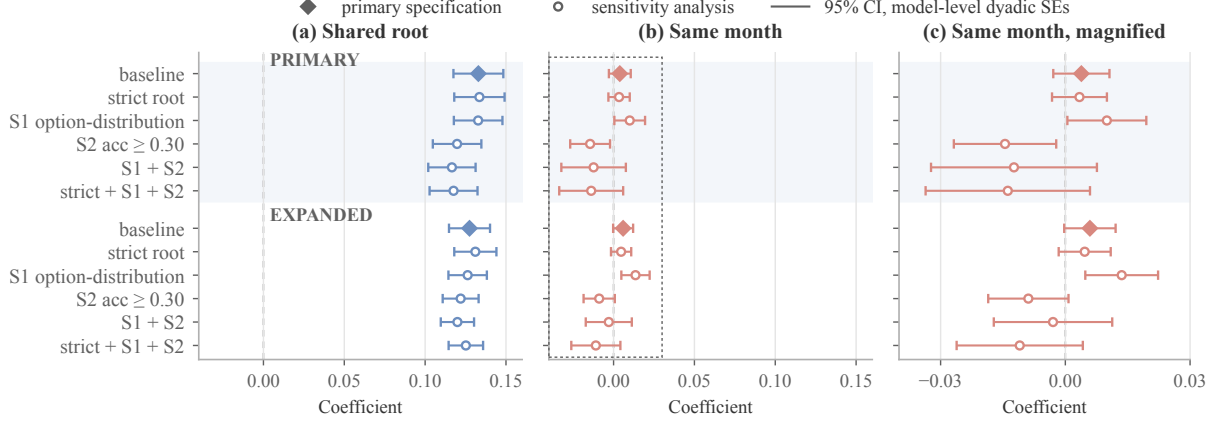
Figure 6. Shared-root and same-month coefficients in the twelve analyses fixed before any pair outcome (model-level dyadic 95% CIs, narrower than the headline jackknife interval of Fig. 10). (a) and (b) share one scale; (c) magnifies the dotted region of (b). Diamonds: primary specifications; values in Table IV.
