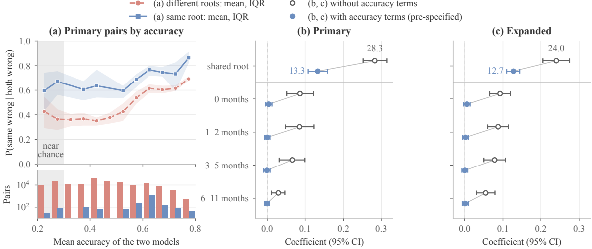
Figure 8. Why accuracy is adjusted for. (a) Mean agreement and interquartile range of primary pairs by their mean accuracy (bins of 0.05 with \geq 30 pairs; 171,735 different-root and 2,020 same-root pairs), with pairs per bin below. (b, c) Coefficients without and with the accuracy terms (jackknife 95% CIs; gaps relative to 12+ months).
