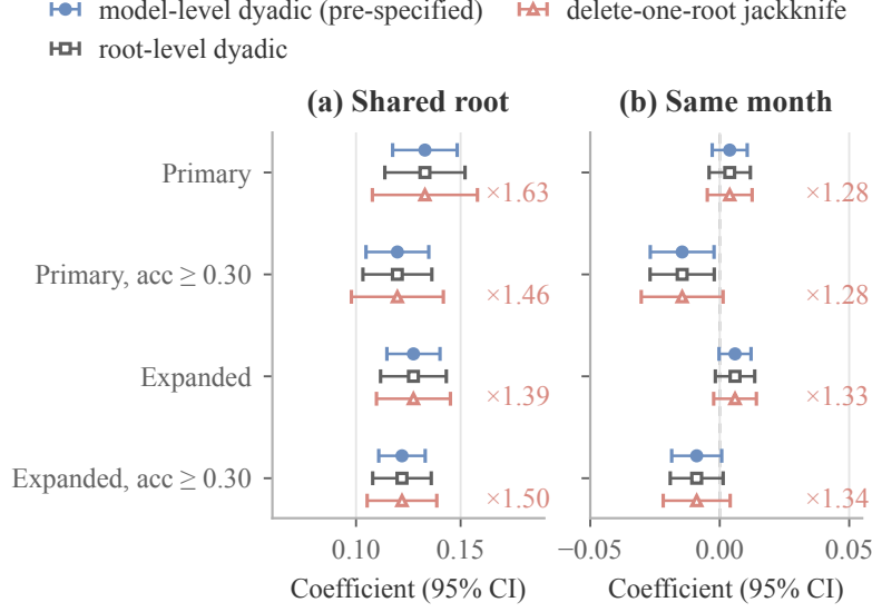
Figure 10. Sensitivity of the intervals to the unit of dependence (95% CIs). Model-level dyadic (pre-specified): pairs sharing a model may be correlated; root-level dyadic: pairs touching a common root; jackknife: one root, with its pairs, omitted at a time. Numbers: jackknife width relative to model-level.
