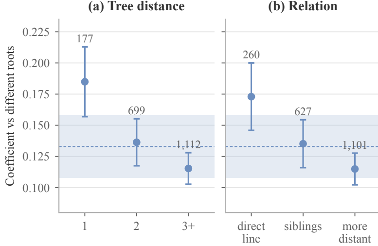
Figure 11. Lineage dose-response (primary sample; in the analysis plan, first run after review; jackknife 95% CIs; labels: pairs). Each coefficient compares one kind of related pair with different-root pairs. Tree distance: declared links through the nearest common ancestor (32 distance-zero pairs not shown). Band and dashed line: the pre-specified shared-root coefficient and interval.
