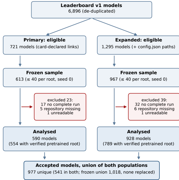
FIGURE 5: Model populations and exclusions. The primary population accepts only lineage links declared on model cards; the expanded population also accepts a model’s first link from its configuration file. Each frozen sample holds at most 40 models per lineage root (seed 0); exclusions are counted per sample, so models in both samples appear in both columns. “Verified pretrained root”: the strict variant used in two pre-specified analyses per population.
