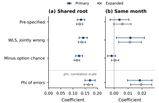
FIGURE 11: Outcome and weighting variants (95% CIs, model-level dyadic). WLS: pairs weighted by the number of jointly wrong items. Minus option chance: agreement minus the agreement expected from the two models' marginal distributions over answer options (exploratory). Phi: the pre-specified secondary outcome, a correlation of error indicators on a different scale. The variant restricted to pairs with at least 1,000 jointly wrong items is identical to the pre-specified fit and is omitted. Values: TABLE VI.
