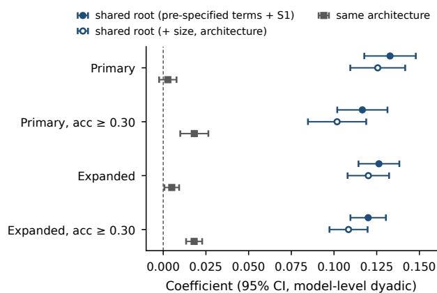
FIGURE 13: Size and architecture controls (exploratory; 95% CIs from model-level dyadic standard errors). Both models include the pre-specified terms and the S1 covariate; the second adds the absolute difference and sum of log parameter counts and a same-architecture indicator. Values: TABLE VIII.
