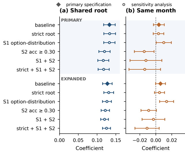
FIGURE 7: Shared-root and same-month coefficients across the twelve pre-specified analyses (95% CIs from model-level dyadic cluster-robust standard errors). Diamonds: the primary specification of each population; open circles: the pre-specified sensitivity analyses. Strict: root verified as a pretrained checkpoint. S1: adds the answer-option-distribution covariate. S2: models with accuracy \geq 0.30 . Note the different horizontal scales: every shared-root interval lies above 0.10, while same-month estimates lie within \pm 0.02 and change sign between specifications. Root-level intervals are in Fig. 10.
