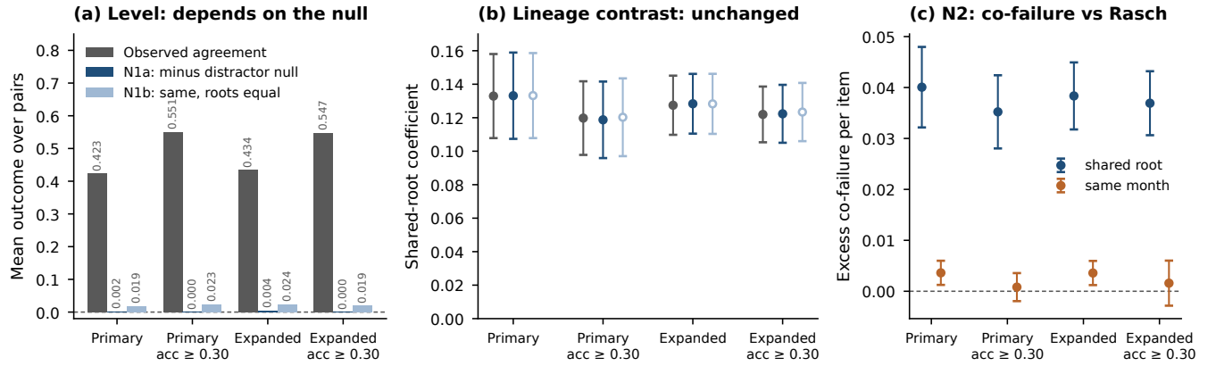
FIGURE 12: Item-difficulty-aware nulls (exploratory, added after review; delete-one-root jackknife 95% CIs). (a) Mean outcome over pairs: observed agreement on wrong answers, and agreement in excess of the item-level distractor null computed from all models (N1a) or with roots weighted equally (N1b). (b) Shared-root coefficient for the same three outcomes. (c) Excess co-failure over a Rasch null (N2), a measure of whether the same items fail, per item: shared-root and same-month coefficients. Values: TABLE VII.
