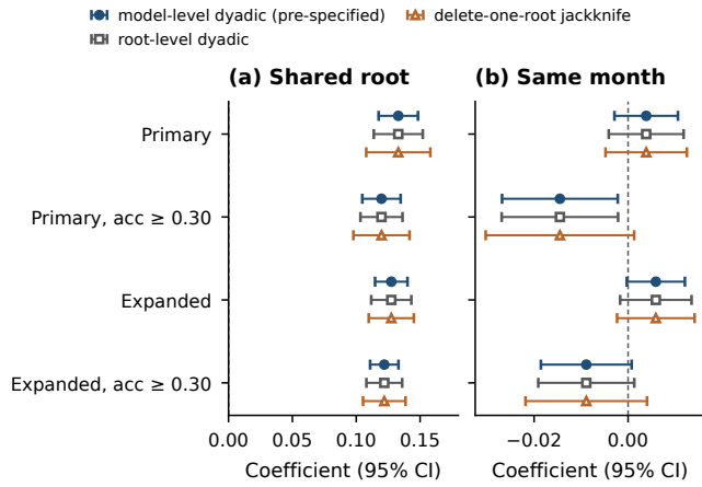
FIGURE 10: Sensitivity of the intervals to the unit of dependence. The pre-specified model-level dyadic intervals allow correlation between pairs sharing a model; root-level dyadic intervals allow it between pairs touching the same lineage root; the jackknife removes one root, and every pair involving it, at a time. Root-level intervals are wider because fine-tunes of one root can err alike in ways not captured by their sharing a model, so the effective number of independent units is closer to the number of roots than of models. Values: TABLE V.
