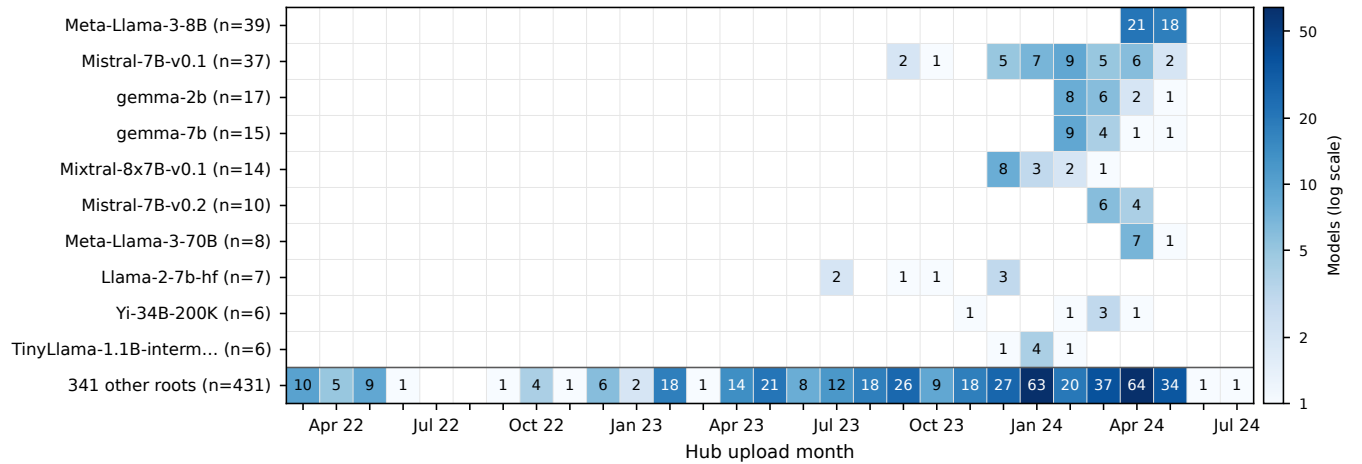
FIGURE 6: Lineage roots by upload month (primary sample, 590 models). Each cell counts the analysed models of one root uploaded in one month (log color scale; empty cells blank). The 10 largest roots are shown individually; the bottom row pools the remaining 341 roots, most of which contribute a single model. Fine-tunes of a root cluster within a few months, so same-root pairs are concentrated at short release-month gaps.
