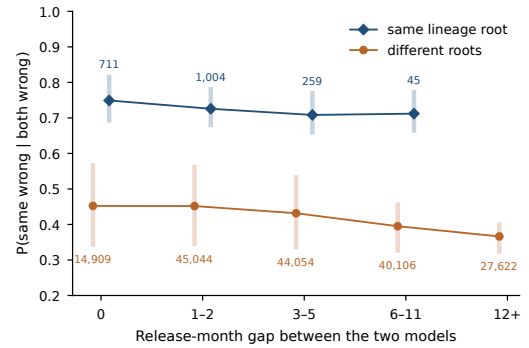
FIGURE 8: Unadjusted agreement on wrong answers by release-month gap for pairs sharing a lineage root and other pairs (primary sample). Points: mean of a_{ij} ; shaded bars: interquartile range across pairs; labels: number of pairs. Bins with fewer than 20 pairs are omitted (one same-root pair is 12 or more months apart). The gap between the two lines is present at every release-month gap; the decline of the lower line with gap is the unadjusted release-time gradient, which is not the adjusted association: it is accounted for by accuracy similarity (Fig. 9).
