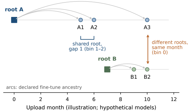
FIGURE 2: The two pair-level predictors (illustration with hypothetical models). Squares are lineage roots and circles fine-tunes placed at their upload month; arcs show declared ancestry. A1 and A2 share a root and were uploaded one month apart (shared root, gap bin 1–2); A3 and B2 descend from different roots but were uploaded in the same month (no shared root, gap bin 0). Every pair carries one value of each predictor, and the pair model estimates each association at equal levels of the other.
