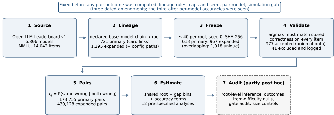
FIGURE 1: Study workflow. Counts are read from the analysis outputs. The primary and expanded samples overlap; 977 is the number of unique accepted models across both. Steps 2–6 were fixed before any pair outcome was computed (three dated amendments, Section III-C); step 7 combines pre-specified secondary analyses with exploratory and post-hoc audits. Primary and expanded populations differ only in the lineage evidence accepted (Section IV-B); a_{ij} is the outcome of Eq. (1).
