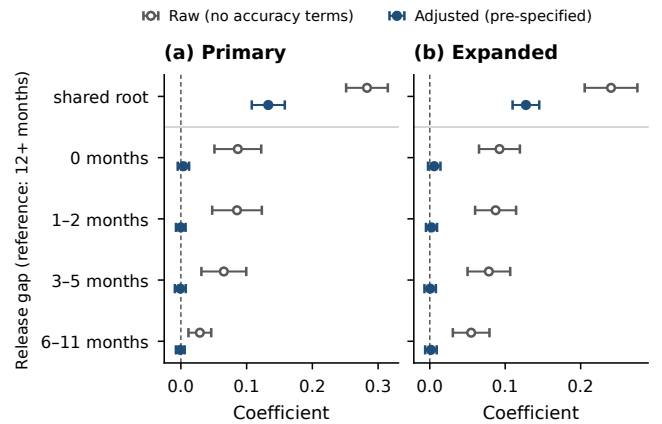
FIGURE 9: Raw and accuracy-adjusted associations (delete-one-root jackknife 95% CIs). Raw: the pre-specified model without the two accuracy terms. Adjusted: the pre-specified model. Release-month bins are relative to the reference category, a gap of 12 or more months. Adding the accuracy terms halves the shared-root coefficient and removes the graded release-time association in both populations. Values: TABLE IV.
