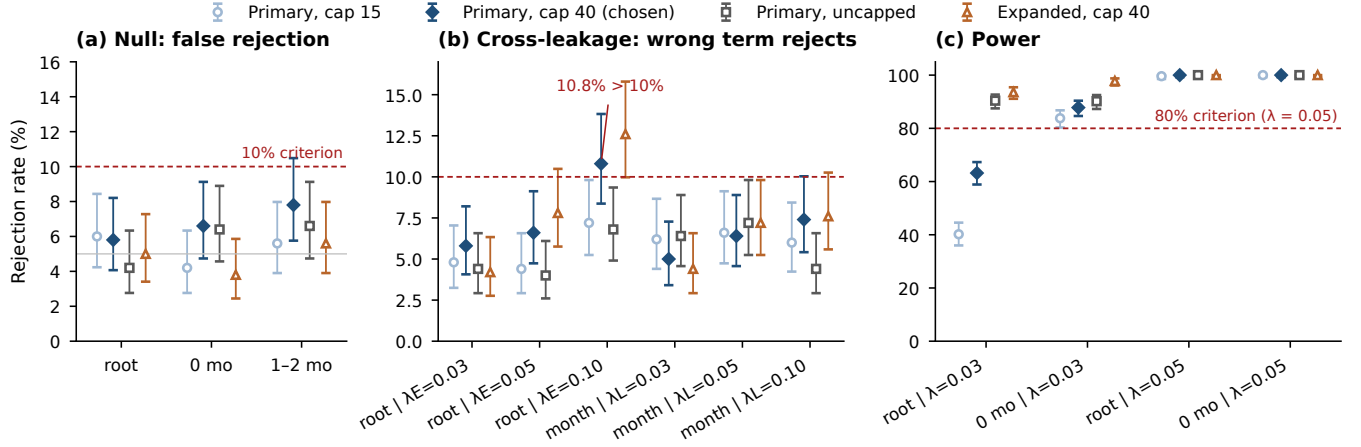
FIGURE 3: Post-hoc audit of the simulation gate (500 replicates per truth; bars are Wilson 95% intervals). (a) Rejection rate of each term when no effect is simulated. (b) Cross-leakage: rejection of the lineage term under release-time-only truths ( \lambda_E ), and of the more often rejecting of the 0- and 1–2-month terms under lineage-only truths ( \lambda_L ). (c) Power of the lineage and same-month terms. Dashed lines mark the pre-specified criteria (10% for null and leakage, 80% for power at \lambda = 0.05 ; no power criterion applied at \lambda = 0.03 ). The chosen design (primary, cap 40) exceeds the leakage criterion at \lambda_E = 0.10 (10.8%, interval 8.4–13.8%), as does the expanded design (12.6%). Not pre-specified.
