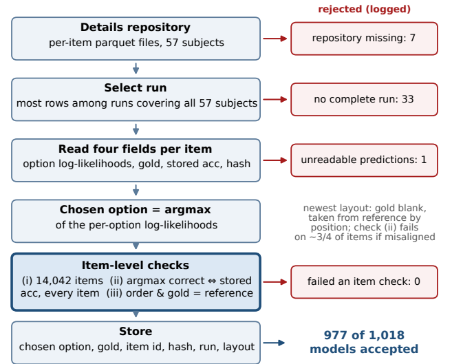
FIGURE 4: Prediction extraction and validation for the 1,018 models in the two frozen samples. Rejections are logged with their reason and were not replaced. Check (ii) compares the argmax of the per-option log-likelihoods with the leaderboard’s stored per-item correctness on every item; no model that reached this step failed it.
