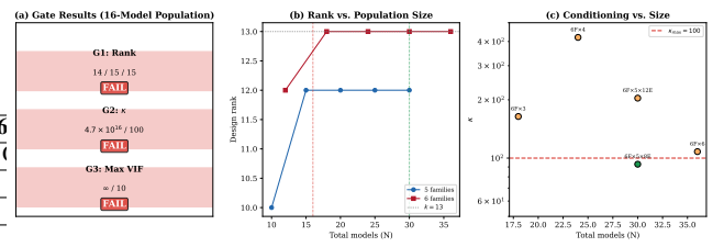
FIGURE 5. Gate diagnostics versus pre-specified thresholds. The 16-model population fails all three gate conditions: rank is 14/15 (G1), condition number is 4.7 \times 10^{16} (G2), and max VIF is infinite (G3).
