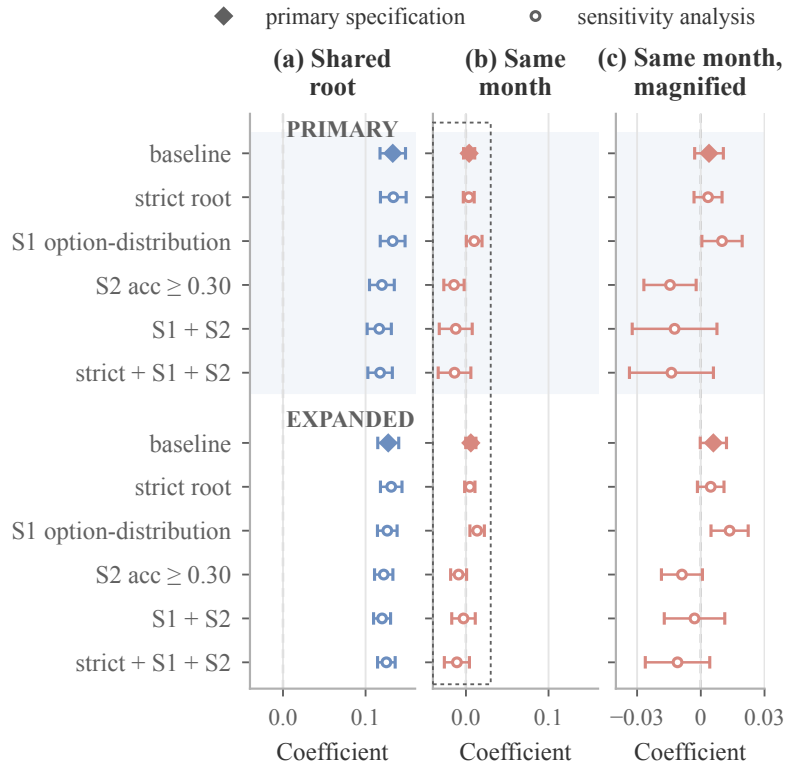
Figure 6. Shared-root and same-month coefficients in the twelve analyses fixed before any pair outcome (95% CIs, model-level dyadic SEs). Panels (a) and (b) share one horizontal scale, so the sizes of the two associations can be compared; panel (c) magnifies the dotted region of (b) on its own scale, so that the sign changes of the same-month coefficient across specifications are visible. Diamonds: the primary specification of each population.
