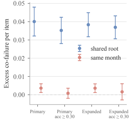
(c) N2: co-failure vs Rasch
