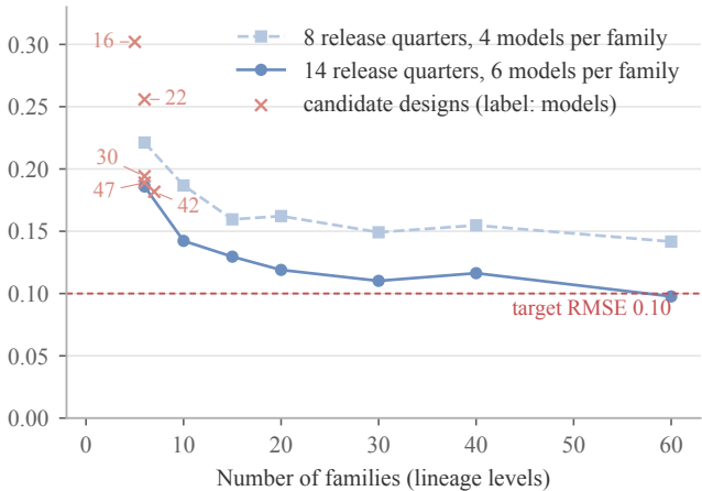
Worst-case RMSE of a variance share
