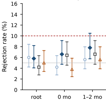
(a) Null: false rejection
