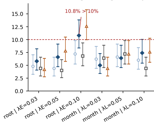
(b) Cross-leakage: wrong term rejects
