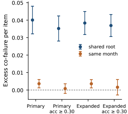
(c) N2: co-failure vs Rasch
