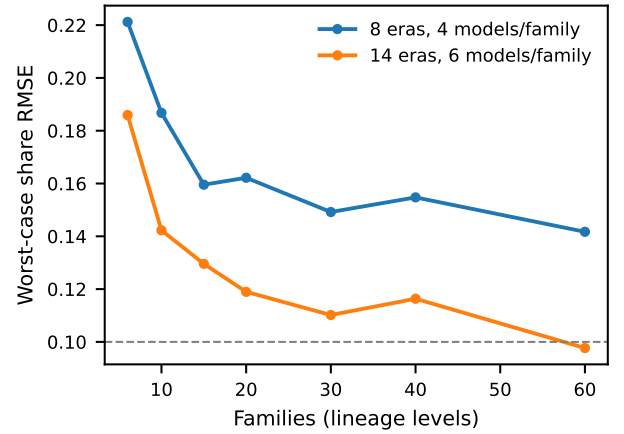
FIGURE 1: Precision of per-model variance shares versus the number of families. Worst-case Monte Carlo RMSE of the family or era share across four scenarios (300 replicates each) for staggered designs. The dashed line marks \pm 0.10 .
