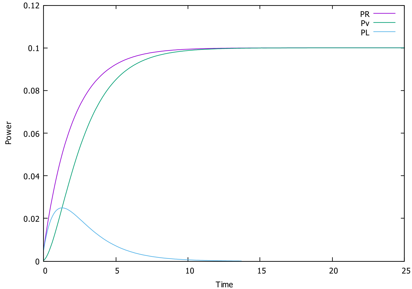
Power in RL Circuit using DC Source
