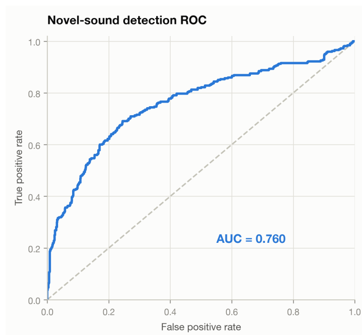
Figure 10: ROC curve for novel-sound detection using autoencoder reconstruction error.
