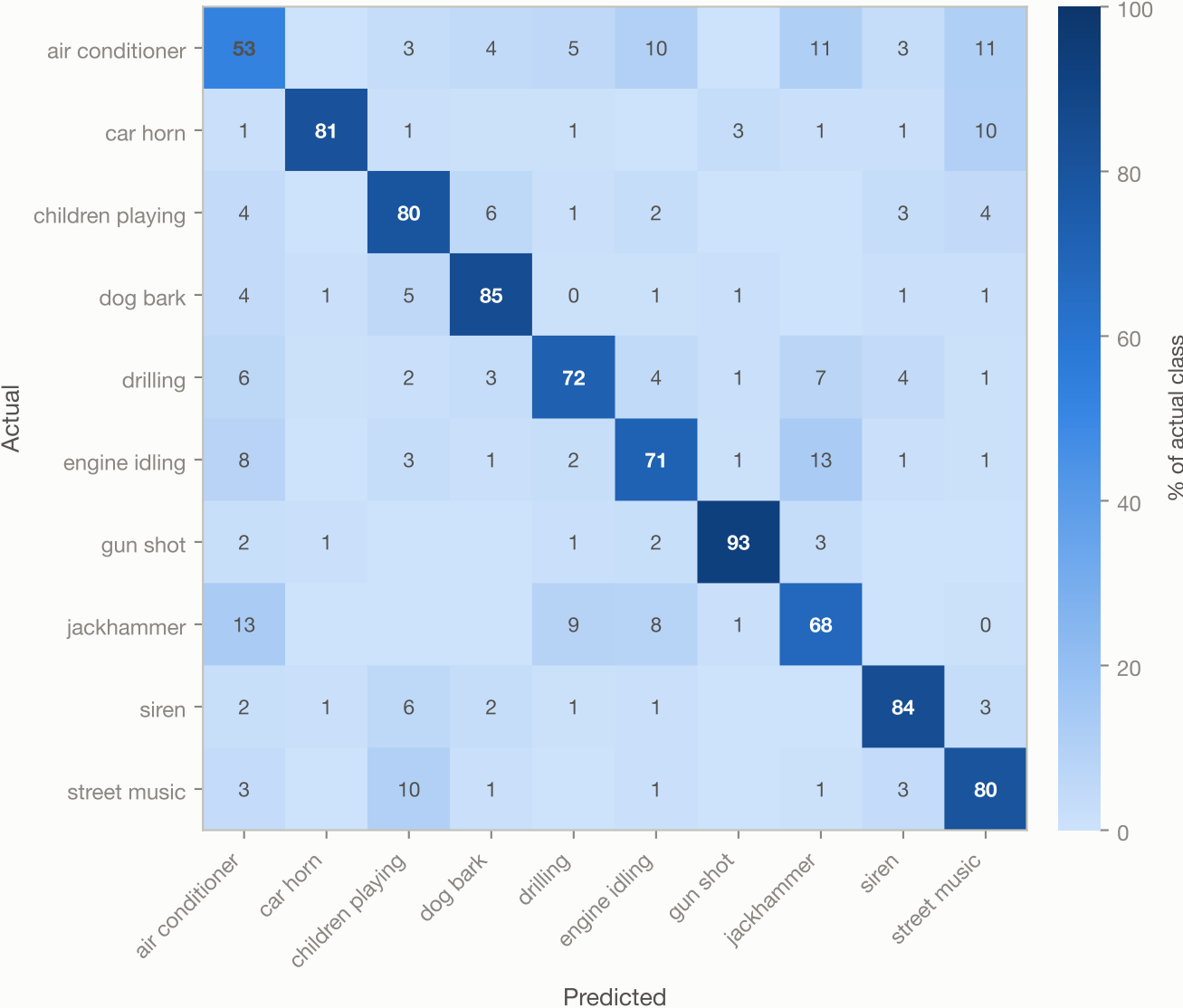
CNN confusion matrix (10-fold aggregate)
