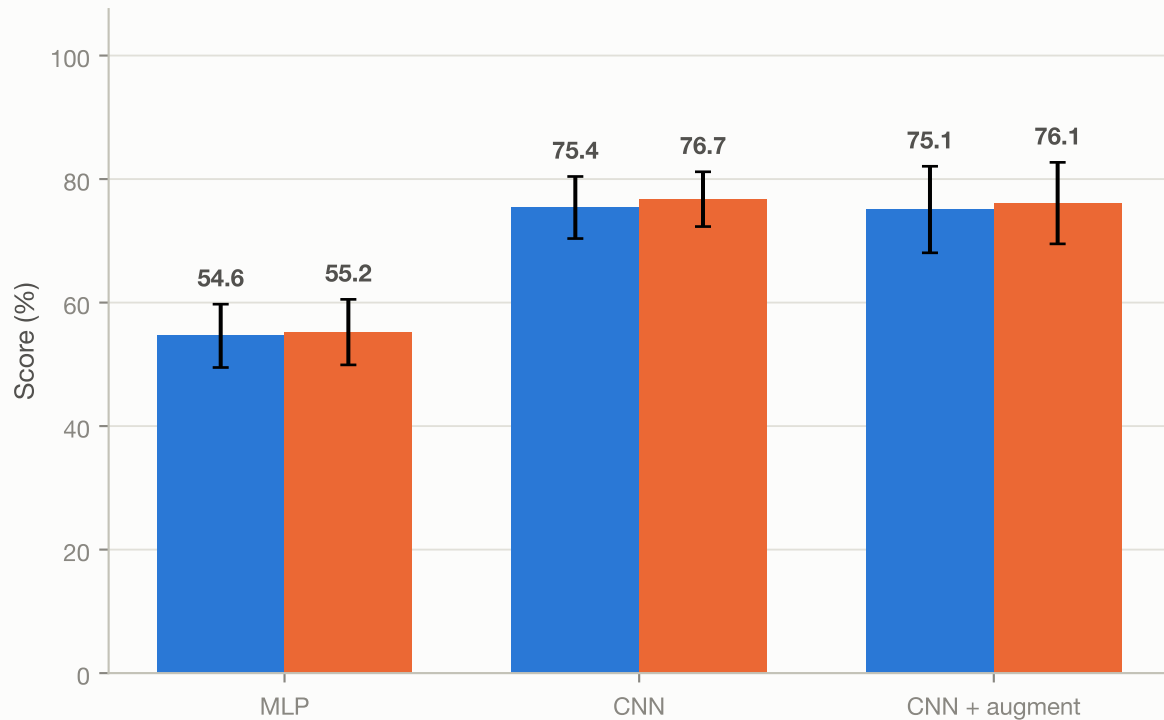
Performance (10-fold mean \pm sd)
