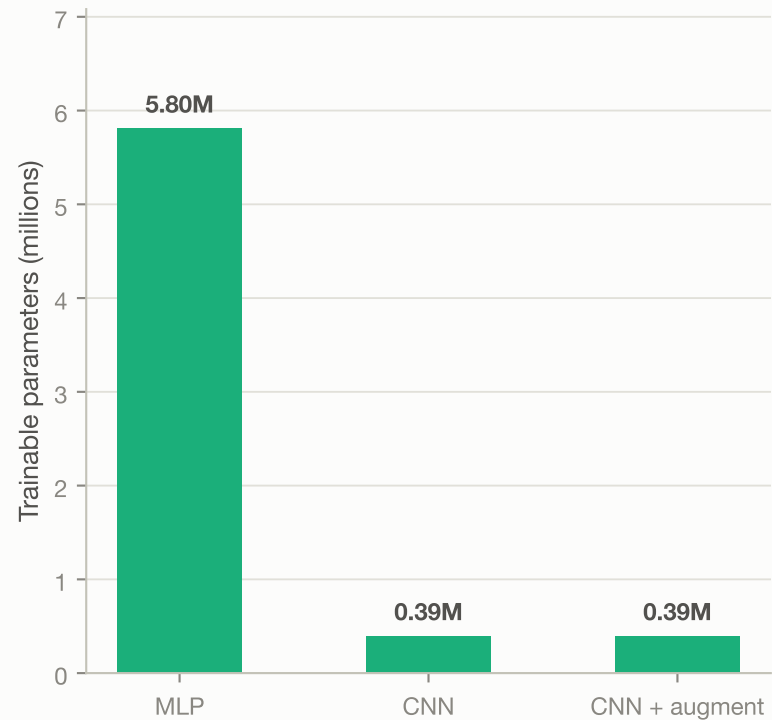
Model size
