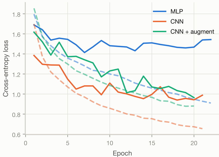
Loss (dashed = train, solid = validation)
