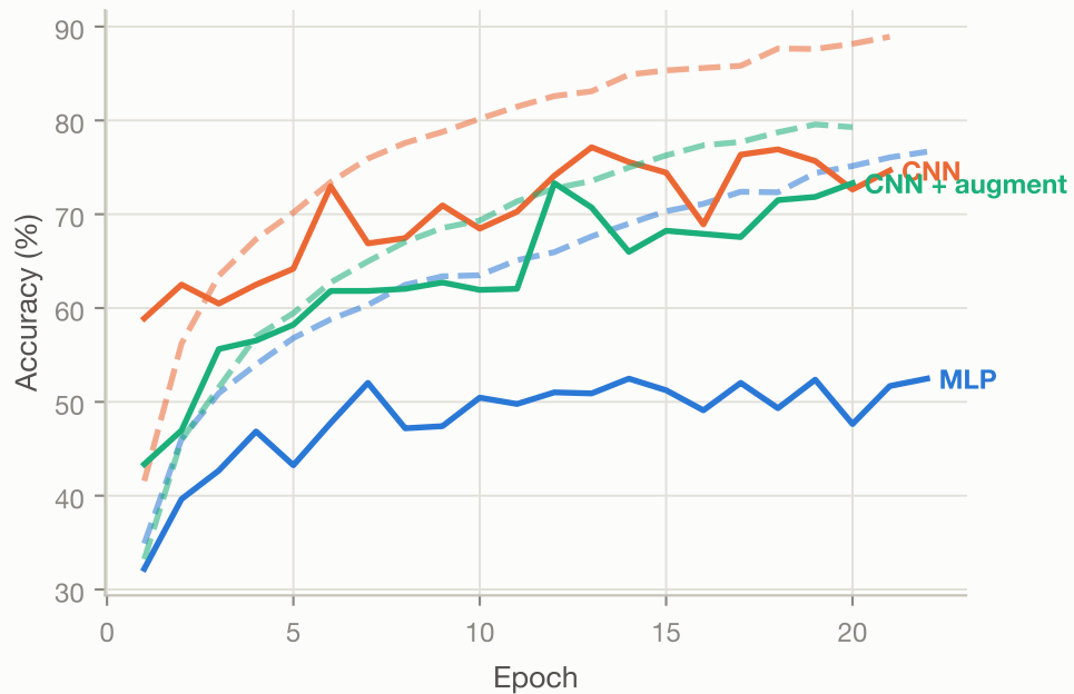
Accuracy (dashed = train, solid = validation)
