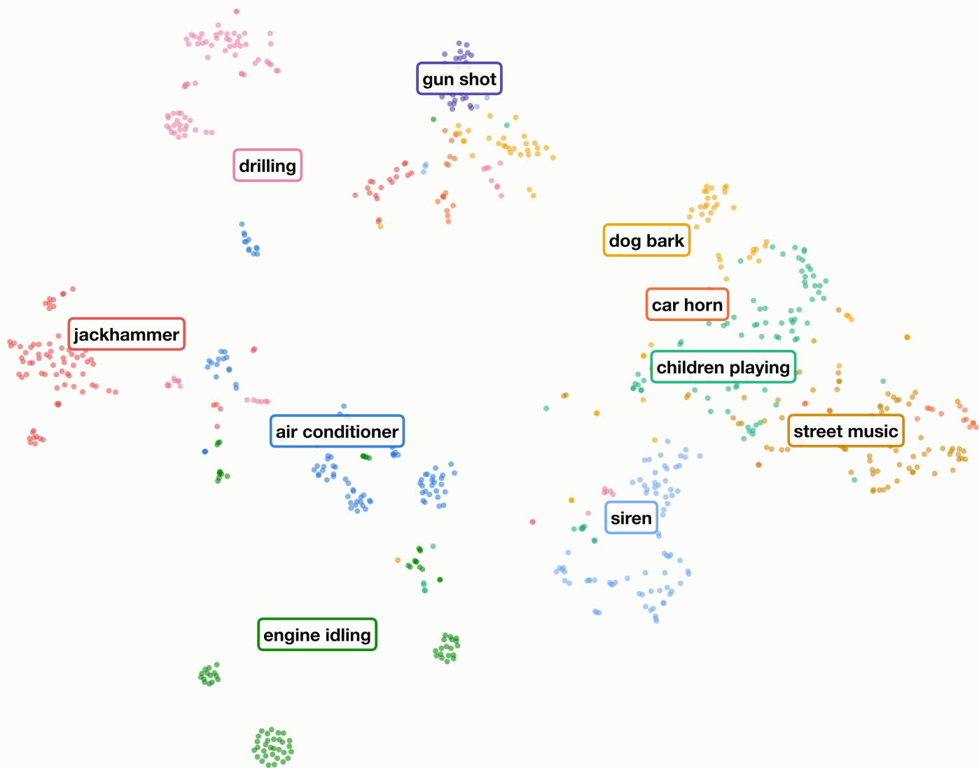
What the CNN learned: t-SNE of 256-d embeddings
