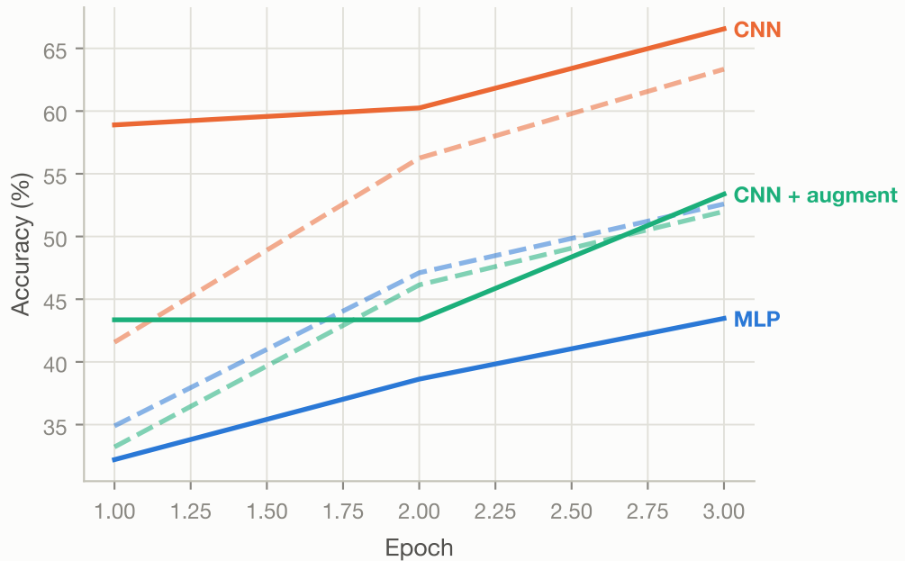
Accuracy (dashed = train, solid = validation)
