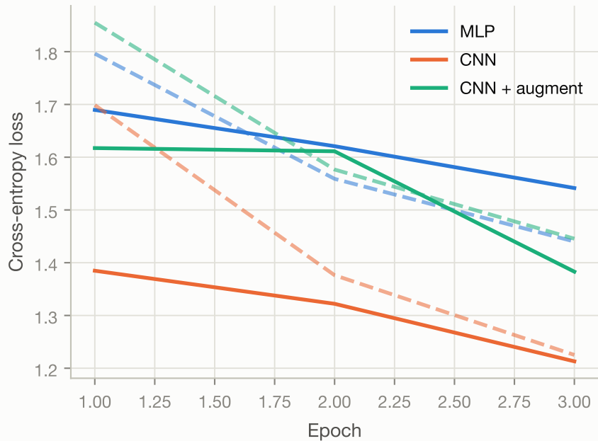
Loss (dashed = train, solid = validation)
