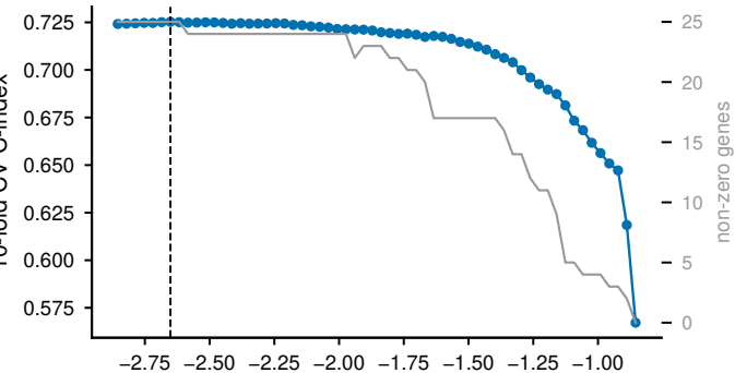
LASSO-Cox regularization path
