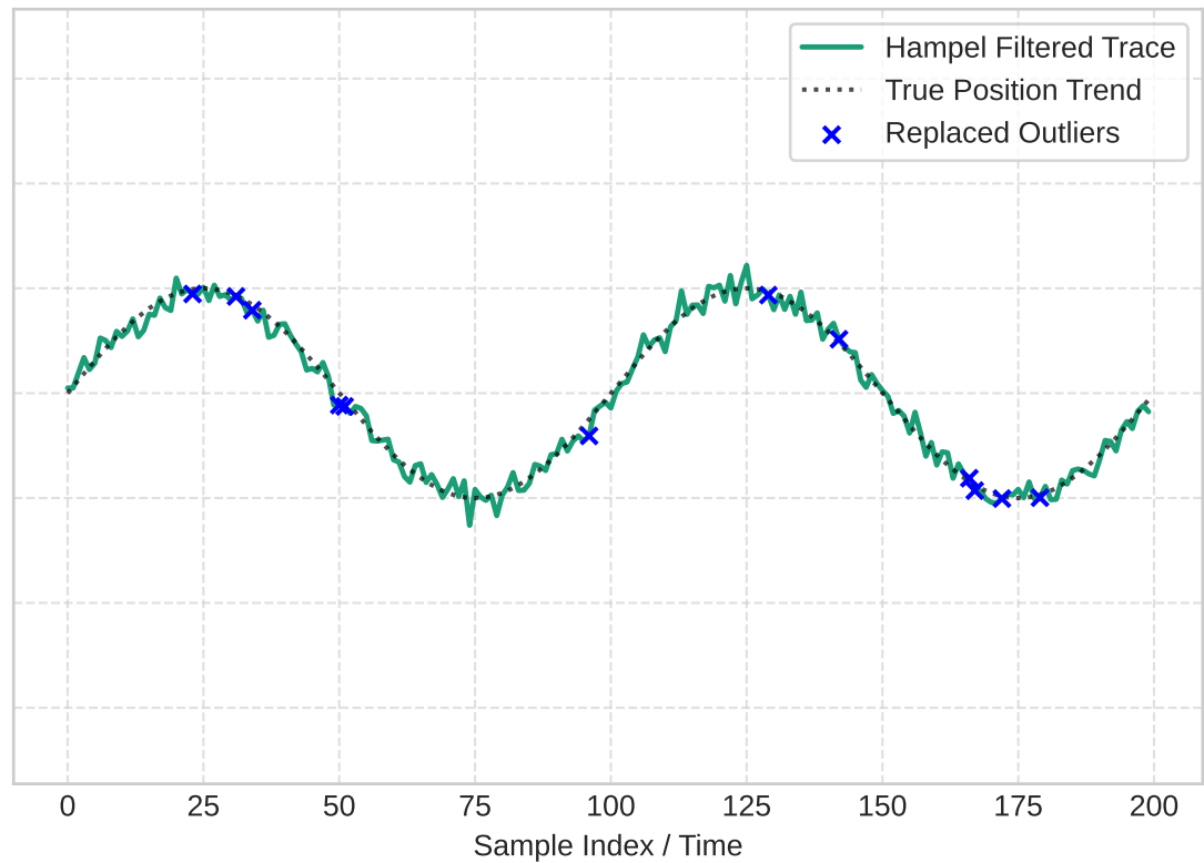
Hampel Filtered CSI Trace ( k = 3.5 )
