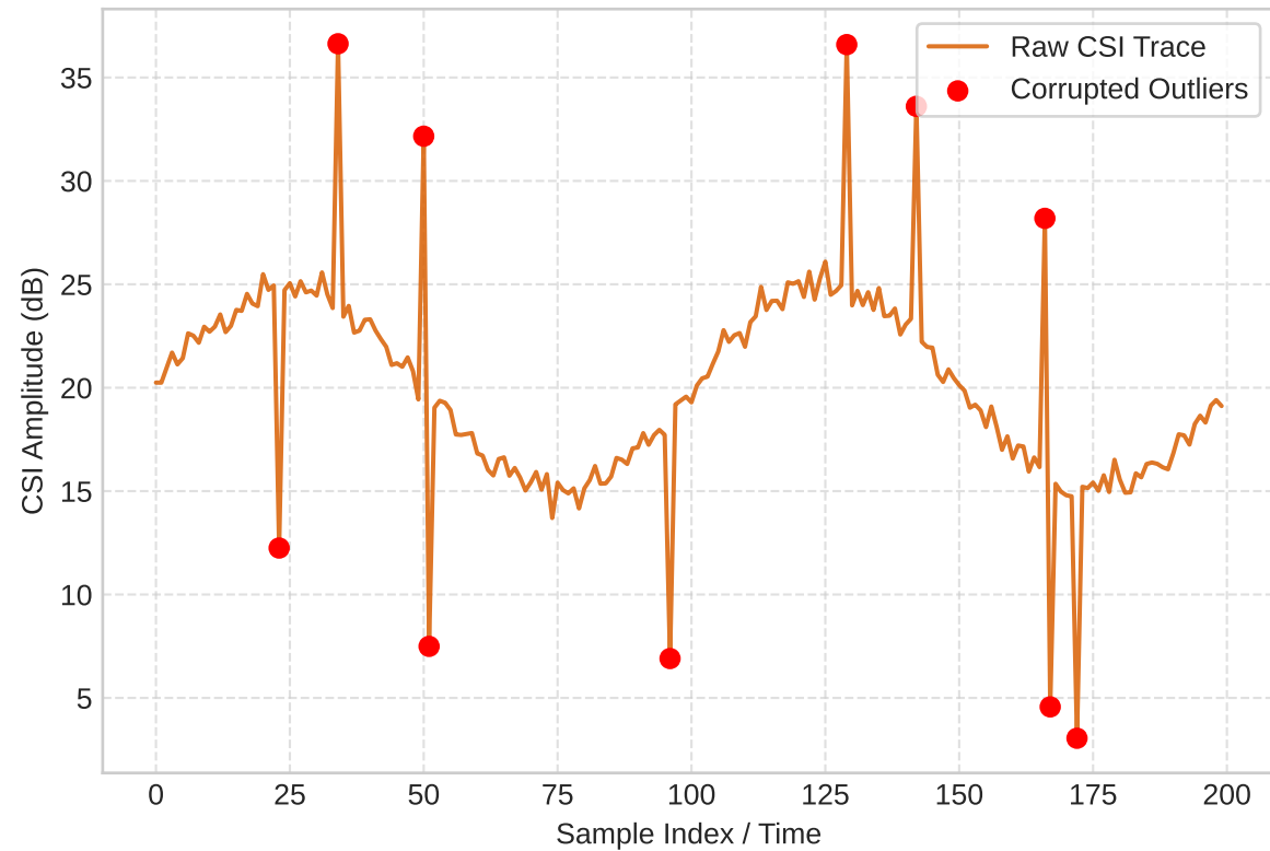
Unfiltered CSI Trace (With Packet Corruptions)
