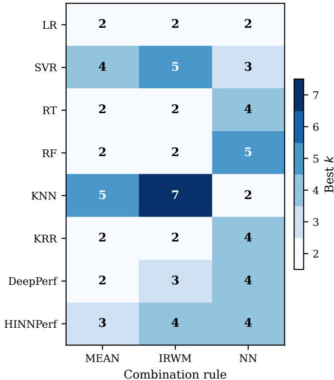
Best k by mean MRE — all scenarios
