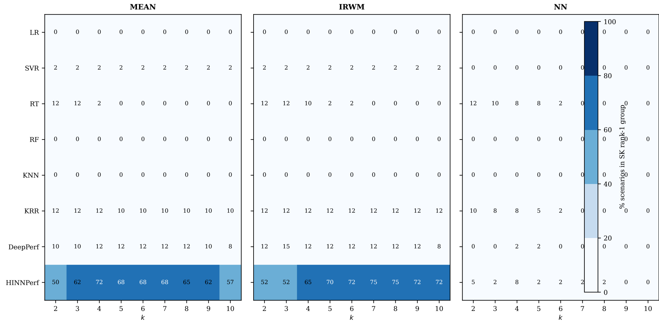
% of scenarios where k is in globally best SK group (all 216 ensembles) — 40 scenarios (RQ3.2)
