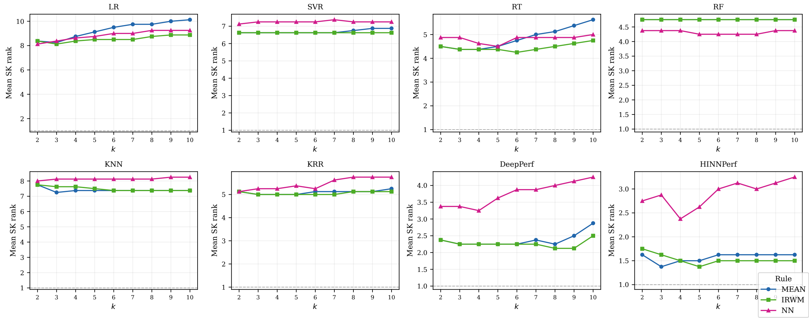
Mean global SK rank vs k — S1 per dataset (RQ3.2) Global competition: all 216 ensembles; dashed line at 1 = globally best group
