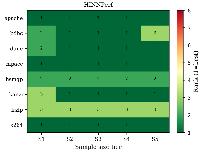
Dataset \times sample-size rank: HINNPerf vs DeepPerf — RQ1
