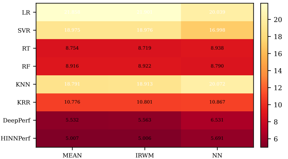
Absolute — MAE
