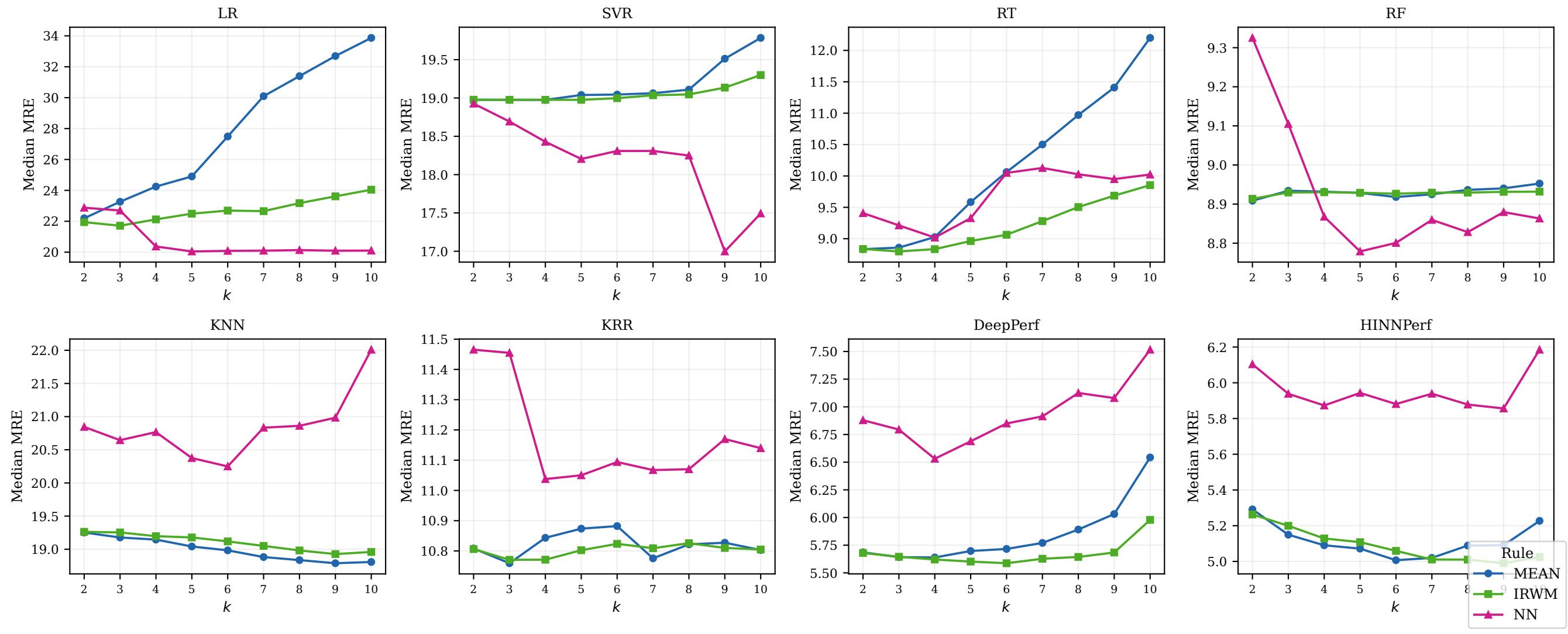
MRE vs. k per base type (median across all 40 scenarios)
