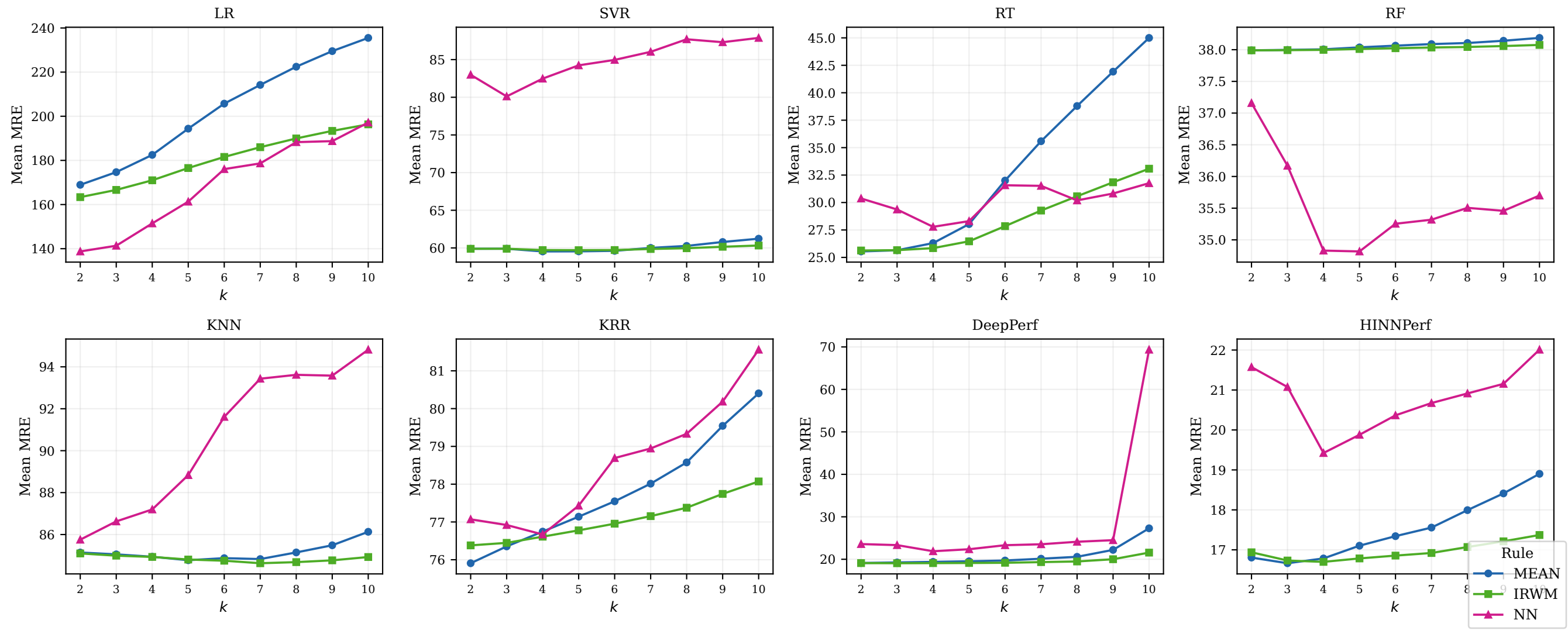
MRE vs. k per base type (mean across all 40 scenarios)
