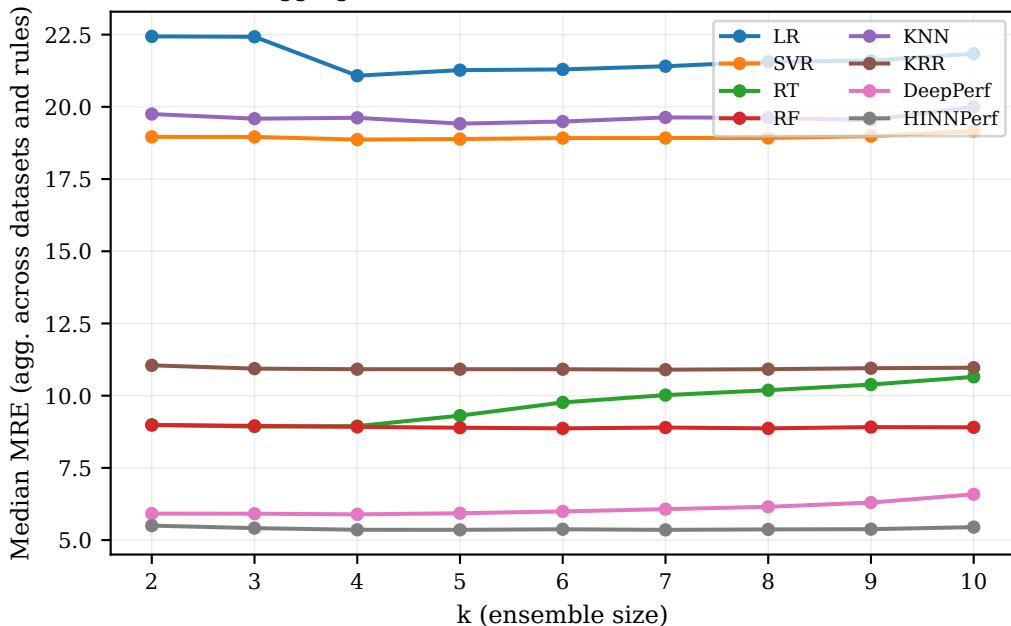
MRE vs k — 1 line per base type, aggregated across all datasets and rules (RQ3.2)
