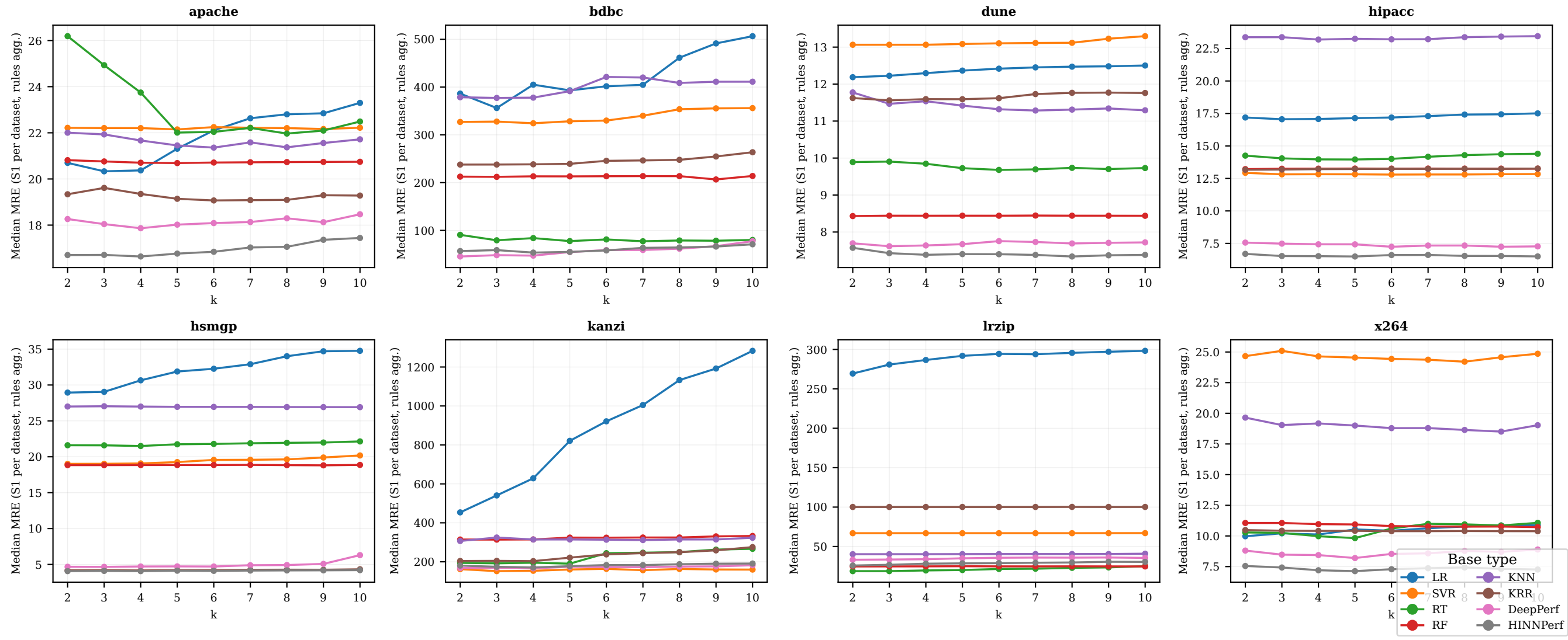
MRE vs k per dataset (S1 per dataset) — 1 line per base type, rules aggregated (RQ3.2)
