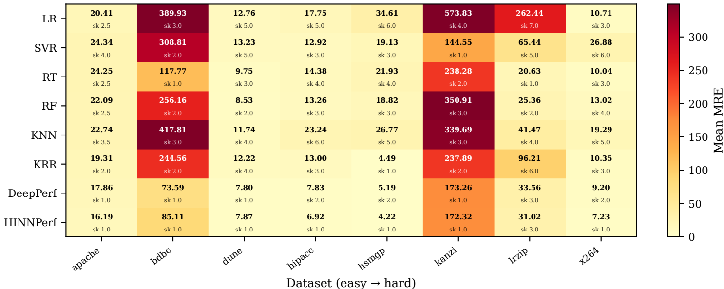
Mean MRE per model × dataset — S1 only (8 scenarios)
