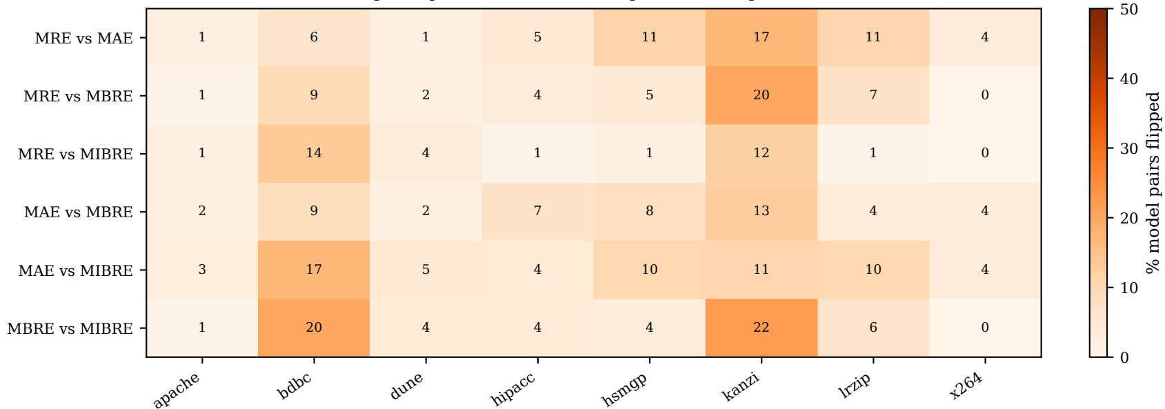
Metric rank-flip rate per dataset — % model pairs that swap relative order (RQ1)
