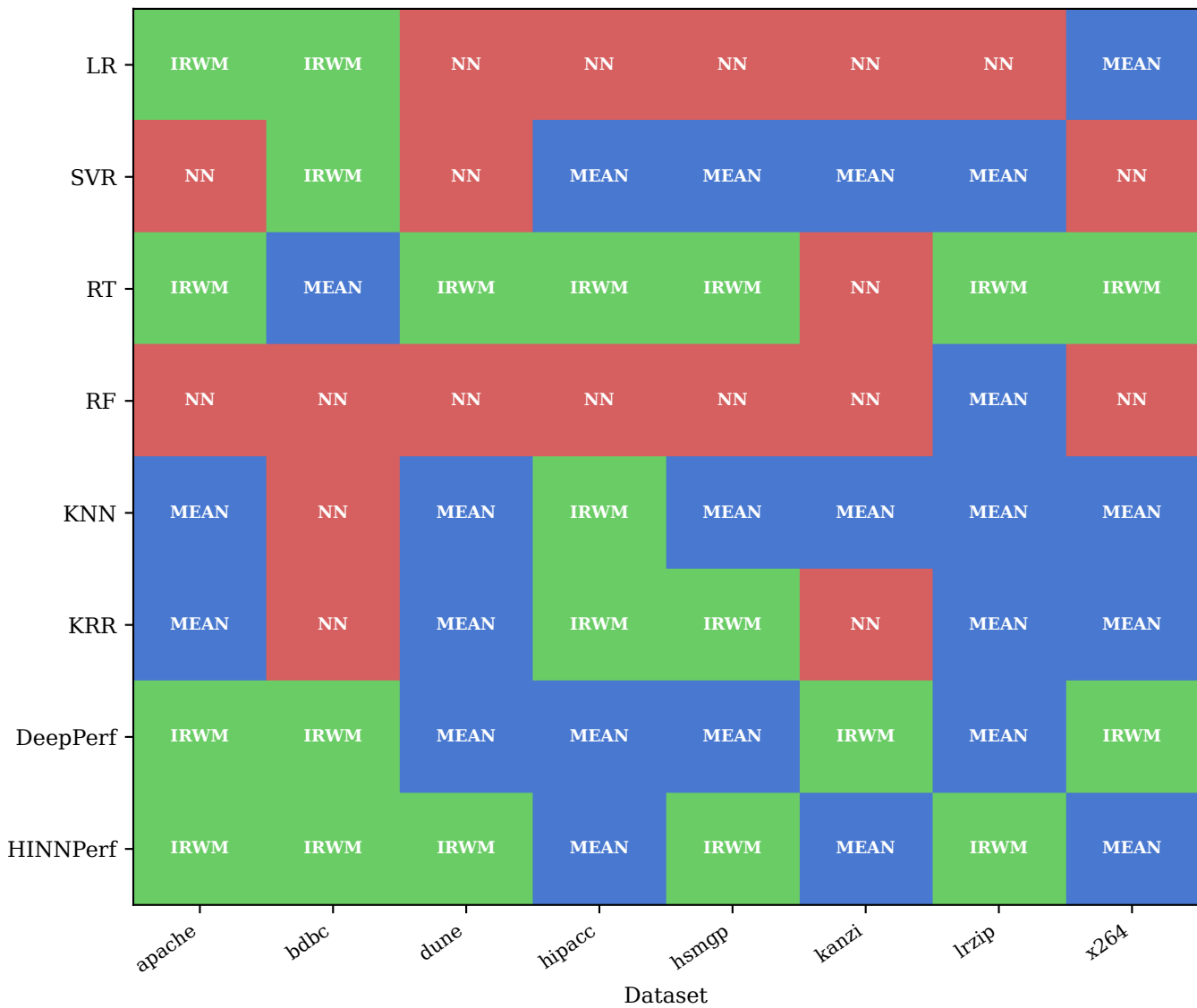
Winning rule per (base type, dataset) — mean MRE, best k per scenario (RQ3.3)
