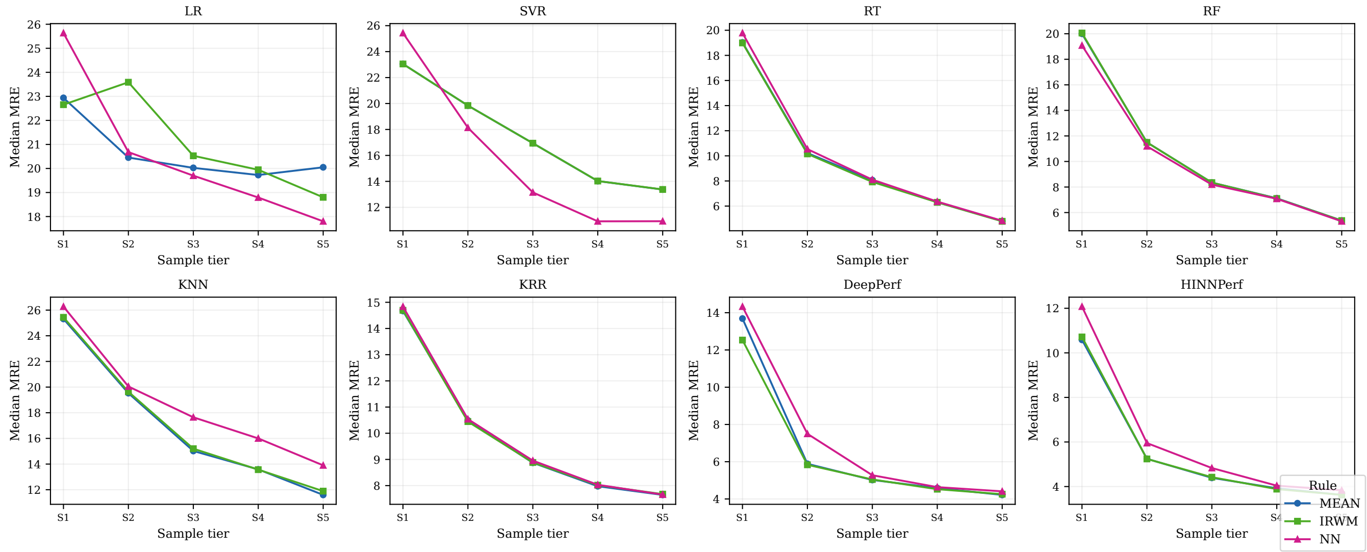
MRE vs. sample size tier per base type — rule comparison (RQ3.3)
