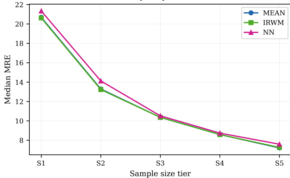
MRE by sample size tier
