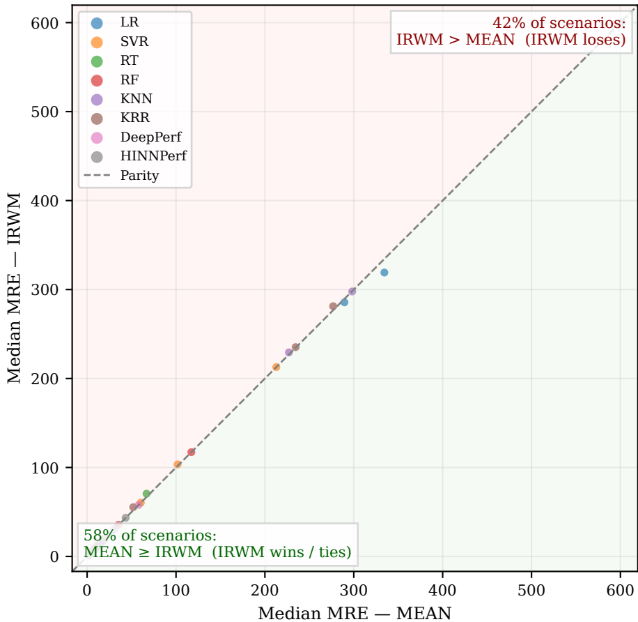
IRWM vs. MEAN: per-scenario MRE (above diagonal = {rule_b} has higher error → {rule_b} loses)
