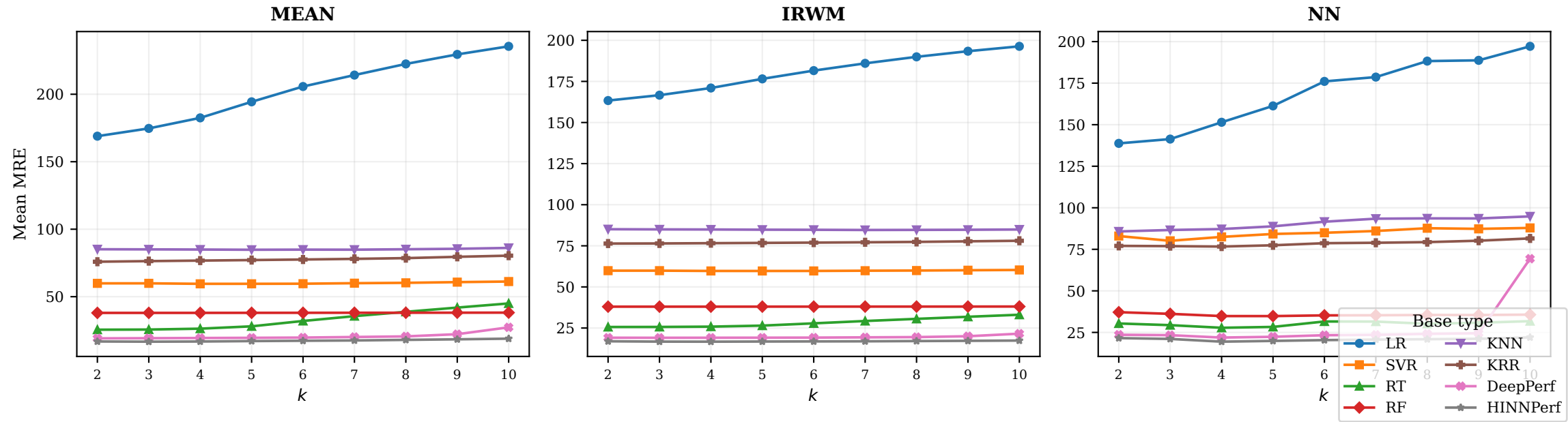
Mean MRE vs. k per rule — 8 base types (all 40 scenarios, RQ3.2)
