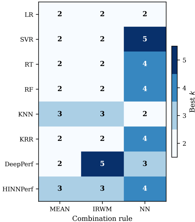
Best k by mean SK rank — S1 only
