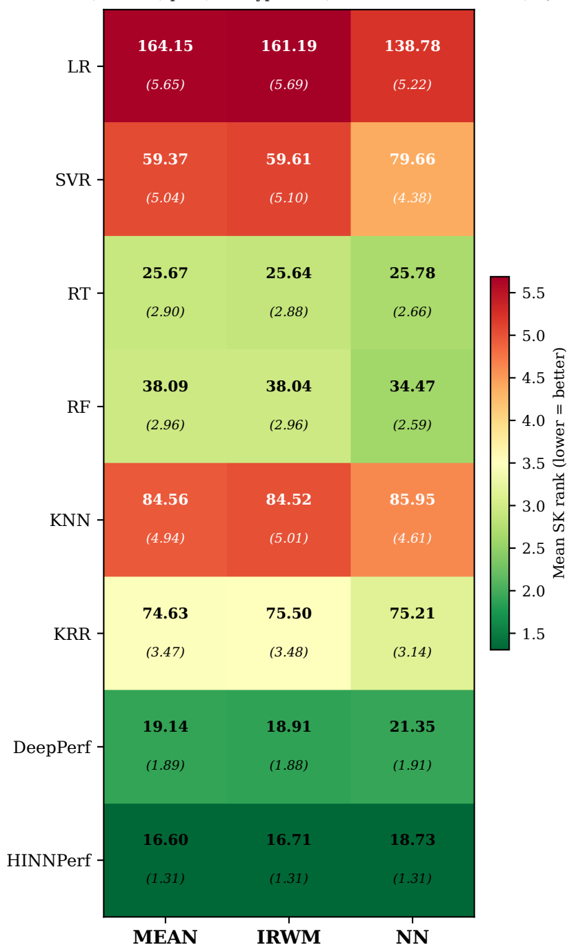
Mean MRE (SK rank) per (base type, rule) — best k , 40 scenarios (RQ3.3)
