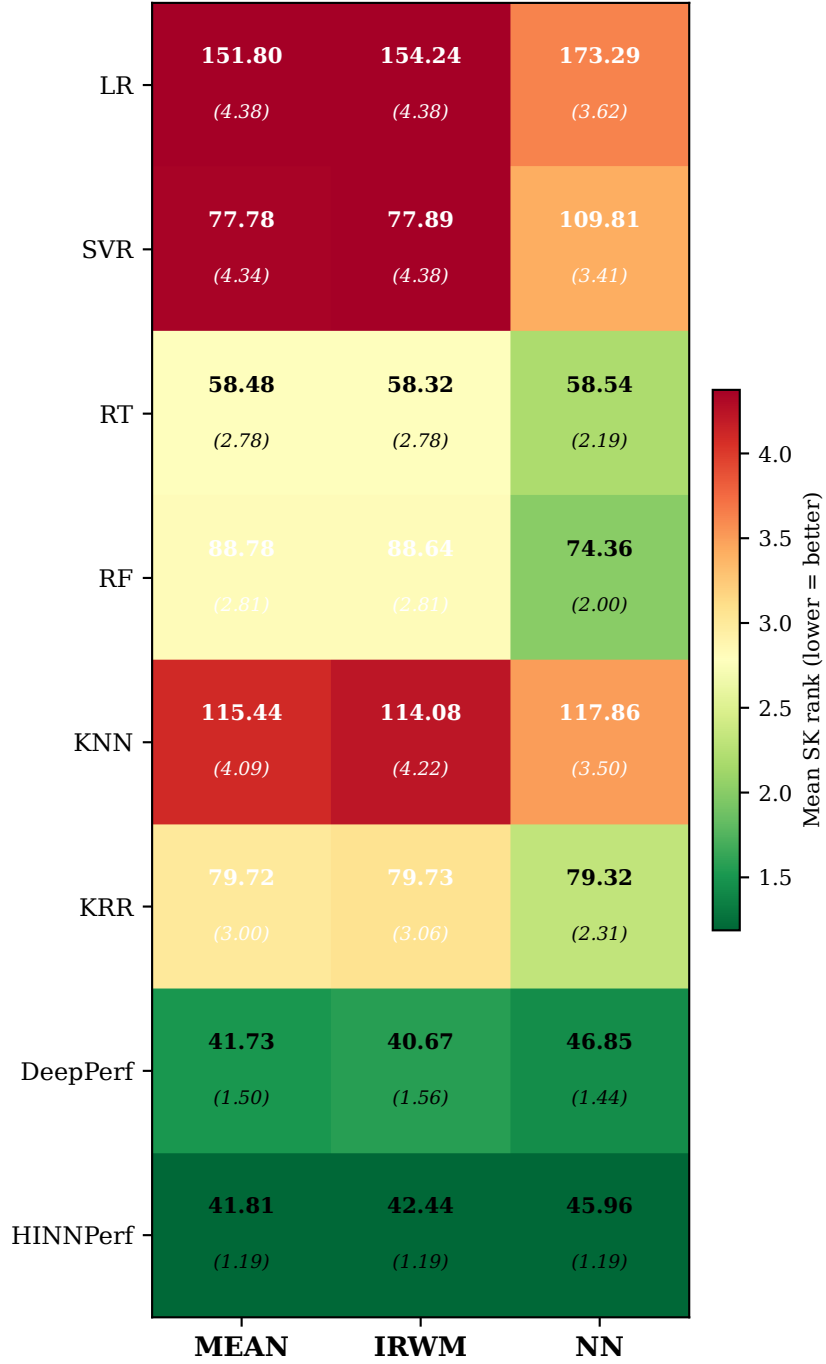
Mean MRE (SK rank) per (base type, rule) — best k , S1 (RQ3.3)
