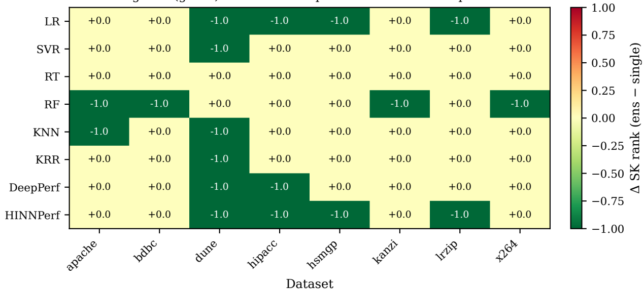
SK rank change: ensemble – single (MRE, S1 per dataset) Negative (green) = ensemble improved at smallest sample size
