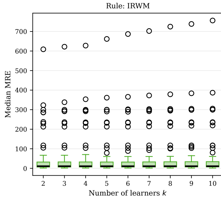
MRE distribution across (base type \times dataset) combos per k
