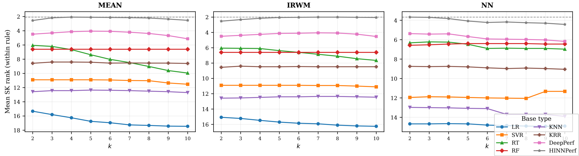
Mean SK rank vs k per rule — 8 base types [global] (all 40 scenarios, RQ3.2)
