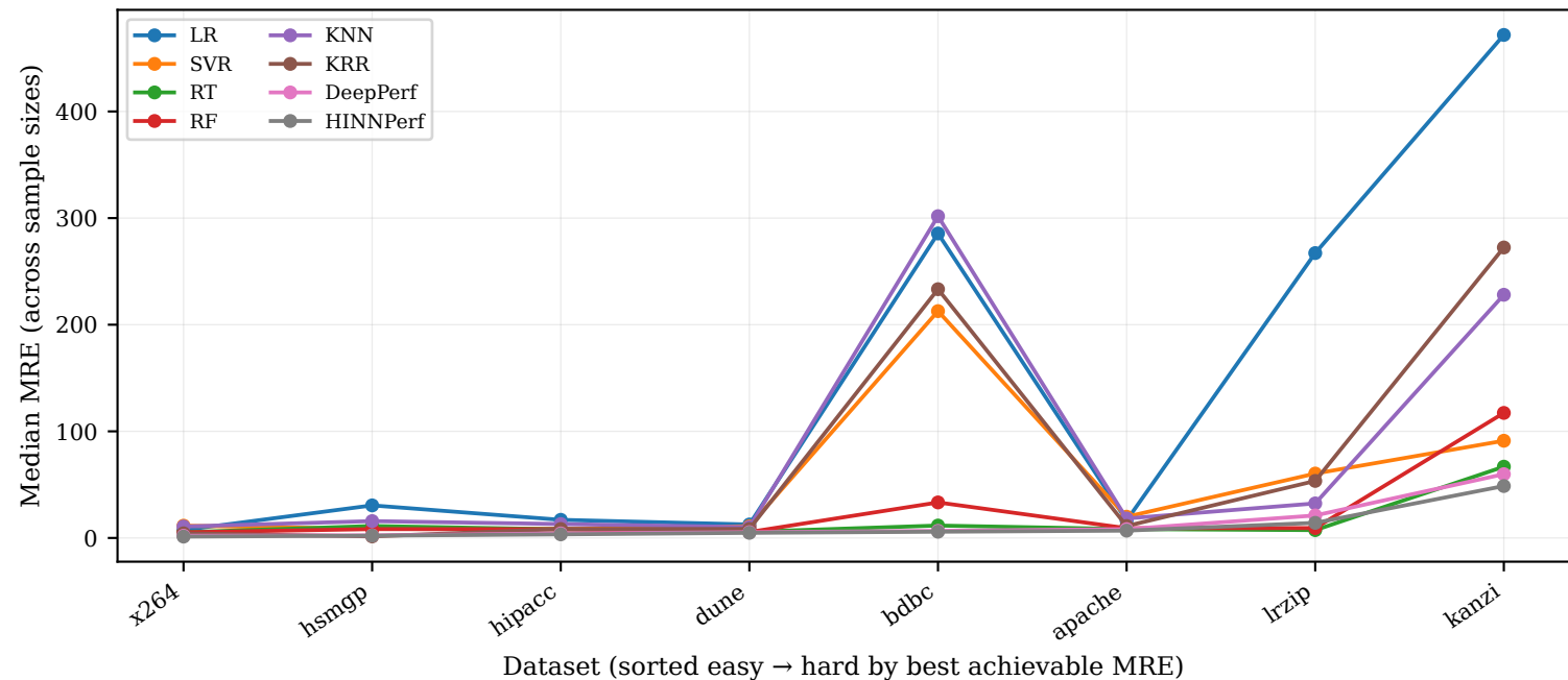
Model performance profiles across datasets — RQ1
